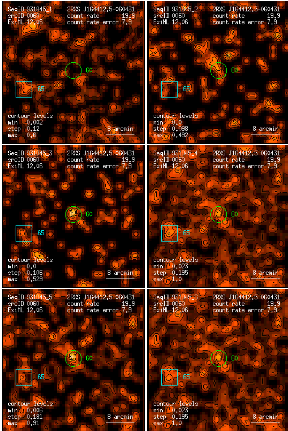
Figure 60: RASS 931845: detection 0060: band rate images, Gaussian filter: (1) PSPC channels 11 – 41, (2) 52 – 90, (3) 91 – 201, (4) 11 – 235, (5) 52 – 201, (6) 11 – 201. Broad band rates in counts/ks. Band rate contour levels in counts/ks/arcmin 2 .
