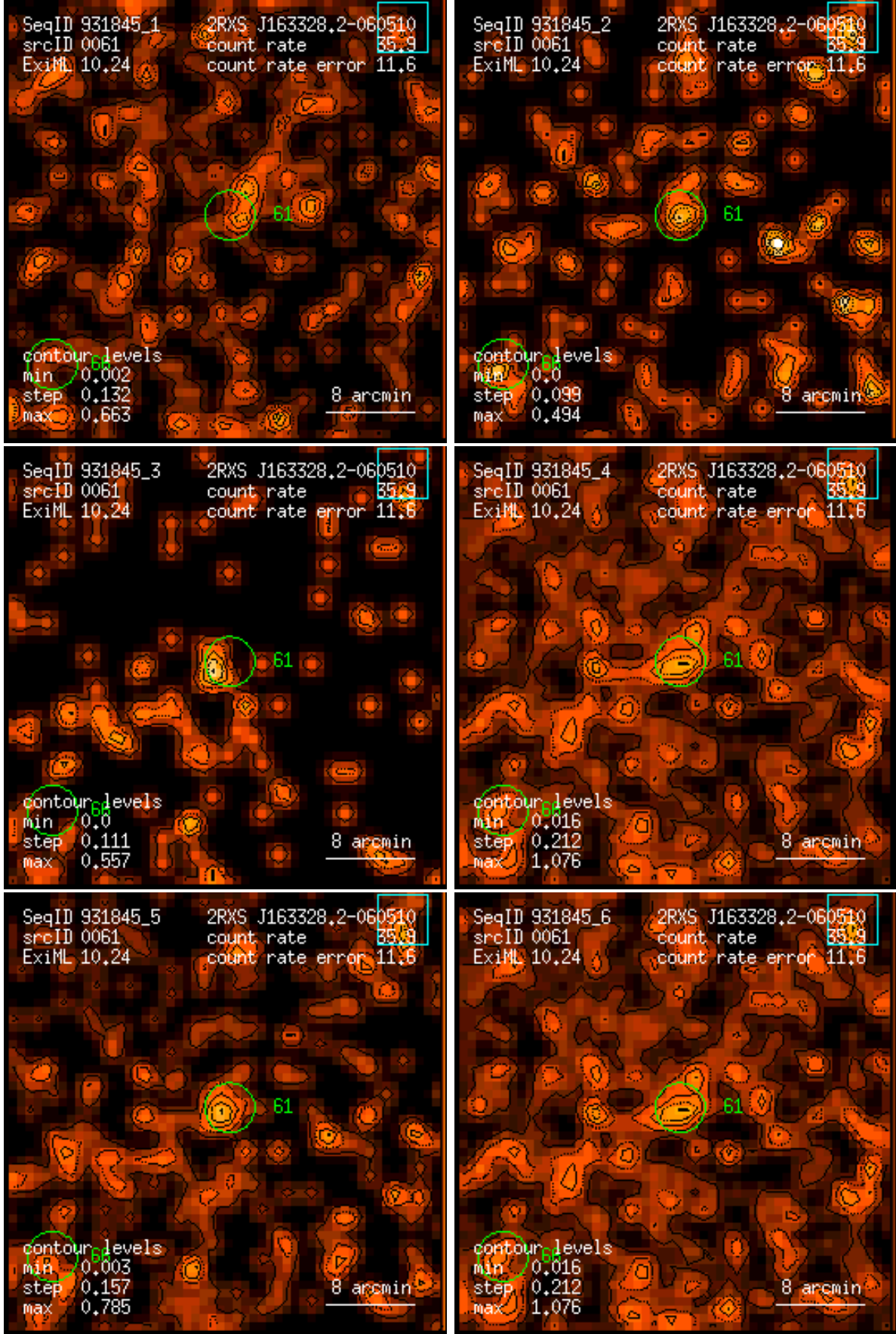
Figure 61: RASS 931845: detection 0061: band rate images, Gaussian filter: (1) PSPC channels 11 – 41, (2) 52 – 90, (3) 91 – 201, (4) 11 – 235, (5) 52 – 201, (6) 11 – 201. Broad band rates in counts/ks. Band rate contour levels in counts/ks/arcmin 2 .
