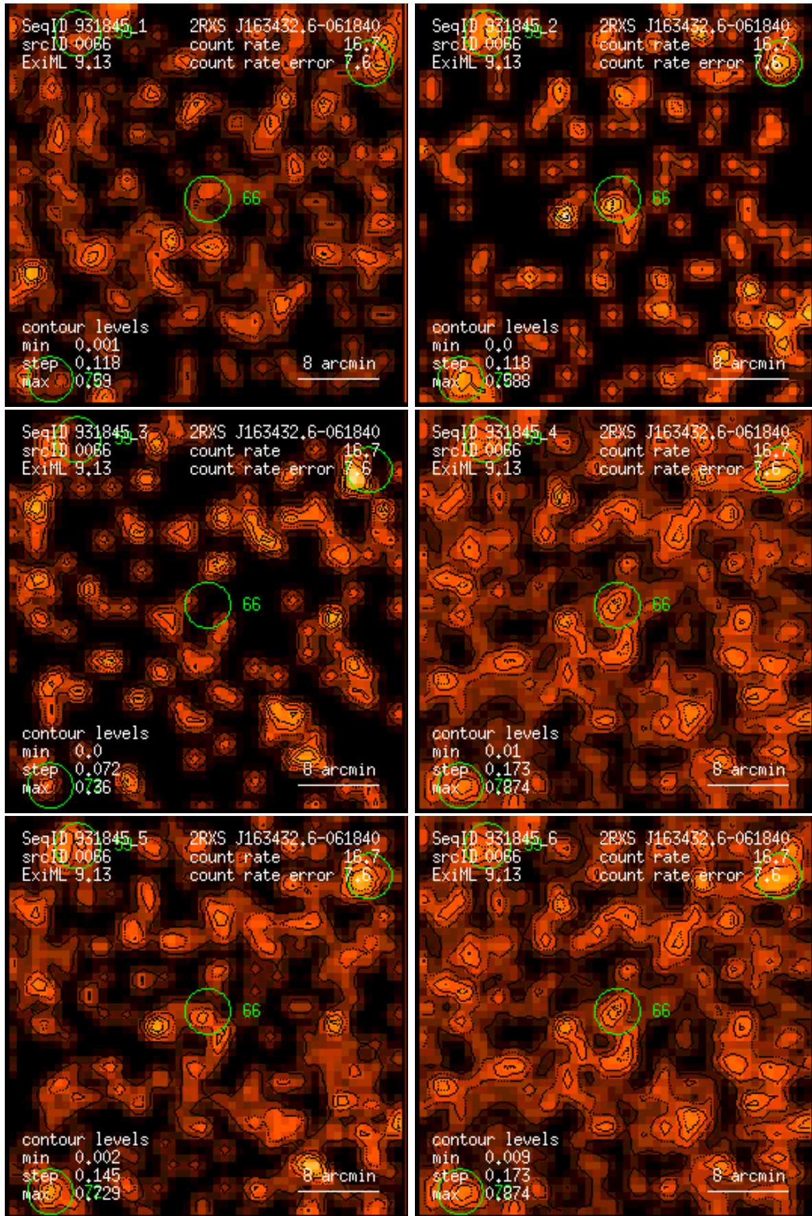
Figure 66: RASS 931845: detection 0066: band rate images, Gaussian filter: (1) PSPC channels 11 – 41, (2) 52 – 90, (3) 91 – 201, (4) 11 – 235, (5) 52 – 201, (6) 11 – 201. Broad band rates in counts/ks. Band rate contour levels in counts/ks/arcmin 2 .
