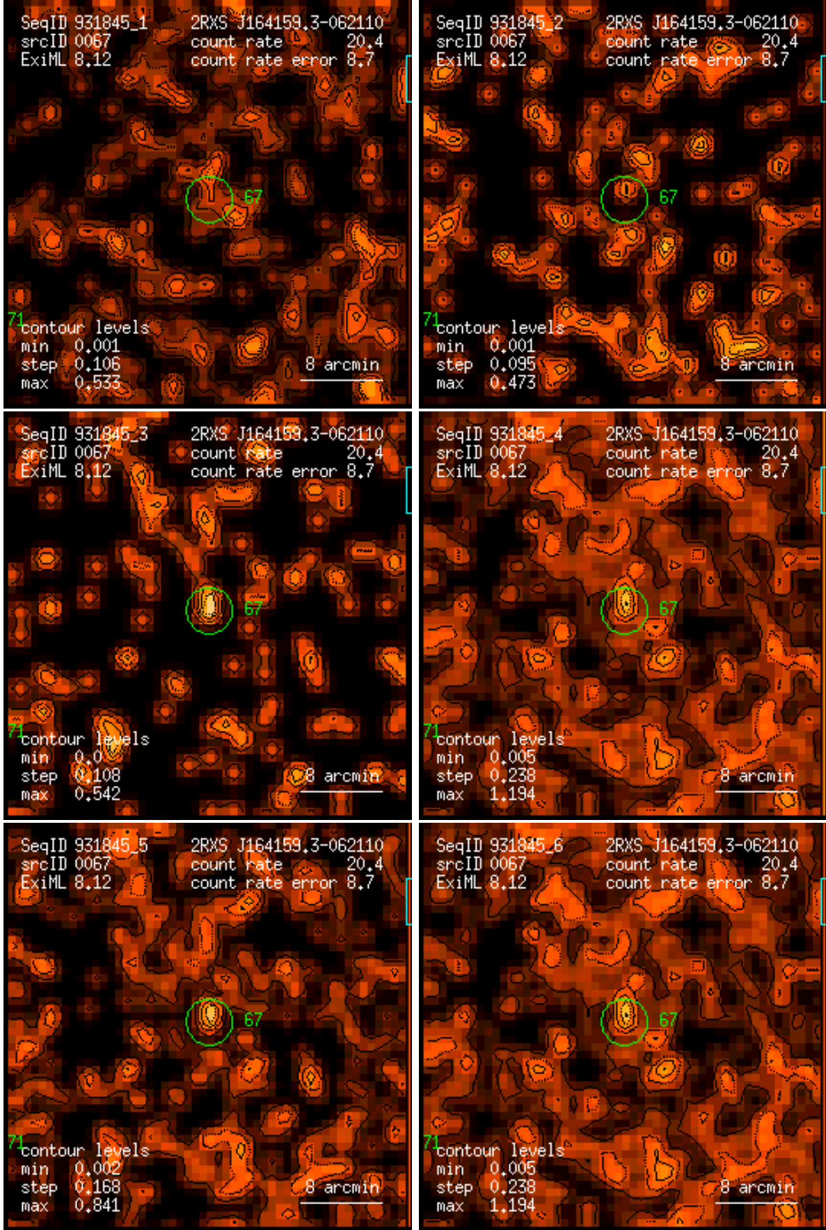
Figure 67: RASS 931845: detection 0067: band rate images, Gaussian filter: (1) PSPC channels 11 – 41, (2) 52 – 90, (3) 91 – 201, (4) 11 – 235, (5) 52 – 201, (6) 11 – 201. Broad band rates in counts/ks. Band rate contour levels in counts/ks/arcmin 2 .
