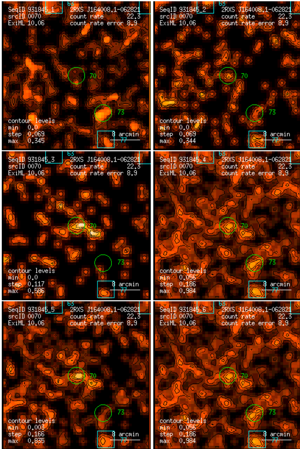
Figure 70: RASS 931845: detection 0070: band rate images, Gaussian filter: (1) PSPC channels 11 – 41, (2) 52 – 90, (3) 91 – 201, (4) 11 – 235, (5) 52 – 201, (6) 11 – 201. Broad band rates in counts/ks. Band rate contour levels in counts/ks/arcmin 2 .
