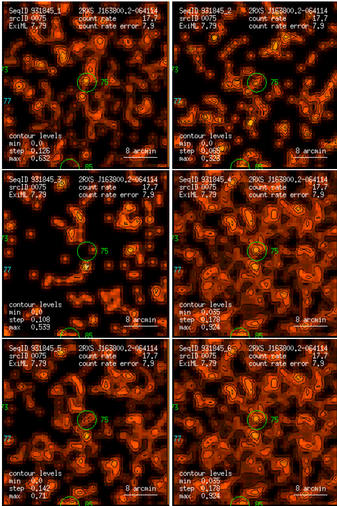
Figure 75: RASS 931845: detection 0075: band rate images, Gaussian filter: (1) PSPC channels 11 – 41, (2) 52 – 90, (3) 91 – 201, (4) 11 – 235, (5) 52 – 201, (6) 11 – 201. Broad band rates in counts/ks. Band rate contour levels in counts/ks/arcmin 2 .
