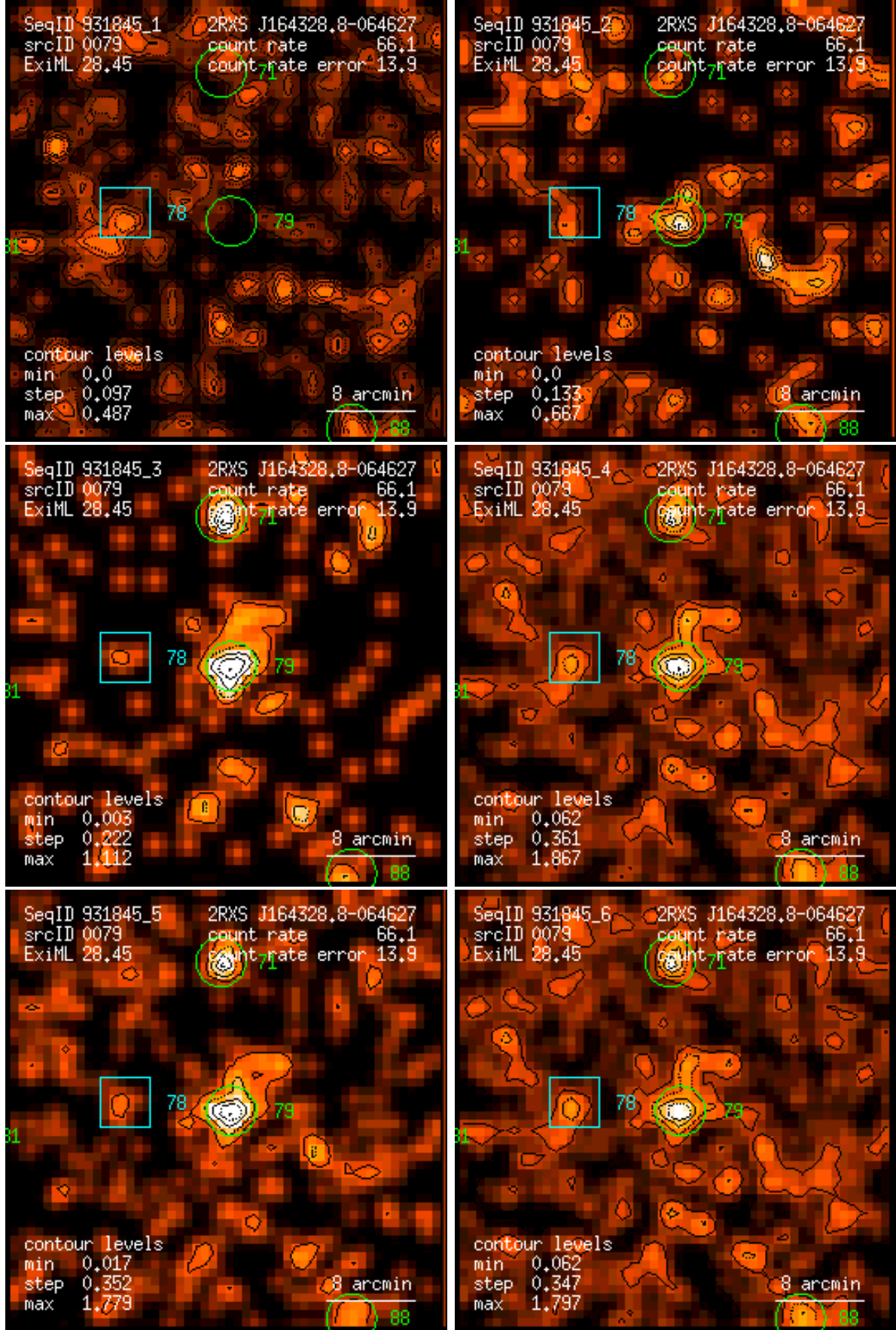
Figure 79: RASS 931845: detection 0079: band rate images, Gaussian filter: (1) PSPC channels 11 – 41, (2) 52 – 90, (3) 91 – 201, (4) 11 – 235, (5) 52 – 201, (6) 11 – 201. Broad band rates in counts/ks. Band rate contour levels in counts/ks/arcmin 2 .
