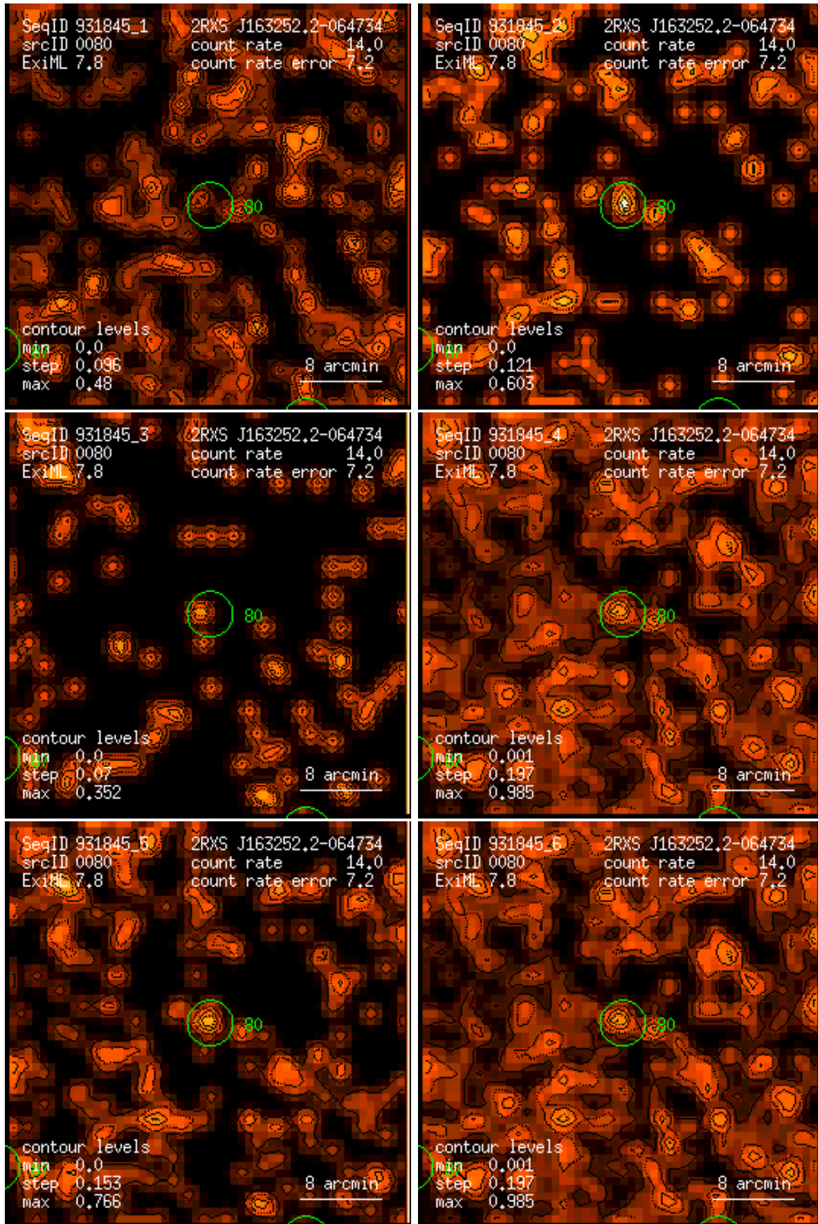
Figure 80: RASS 931845: detection 0080: band rate images, Gaussian filter: (1) PSPC channels 11 – 41, (2) 52 – 90, (3) 91 – 201, (4) 11 – 235, (5) 52 – 201, (6) 11 – 201. Broad band rates in counts/ks. Band rate contour levels in counts/ks/arcmin 2 .
