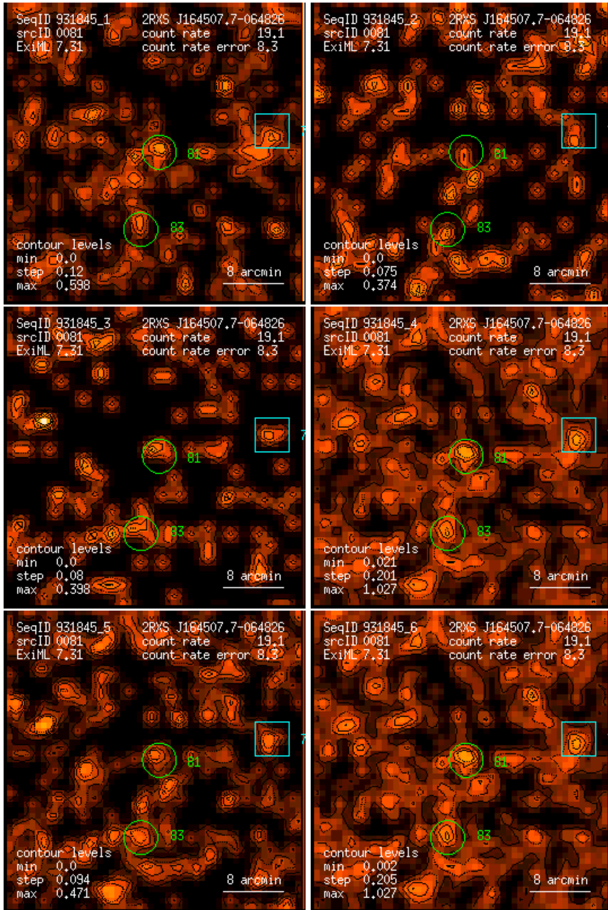
Figure 81: RASS 931845: detection 0081: band rate images, Gaussian filter: (1) PSPC channels 11 – 41, (2) 52 – 90, (3) 91 – 201, (4) 11 – 235, (5) 52 – 201, (6) 11 – 201. Broad band rates in counts/ks. Band rate contour levels in counts/ks/arcmin 2 .
