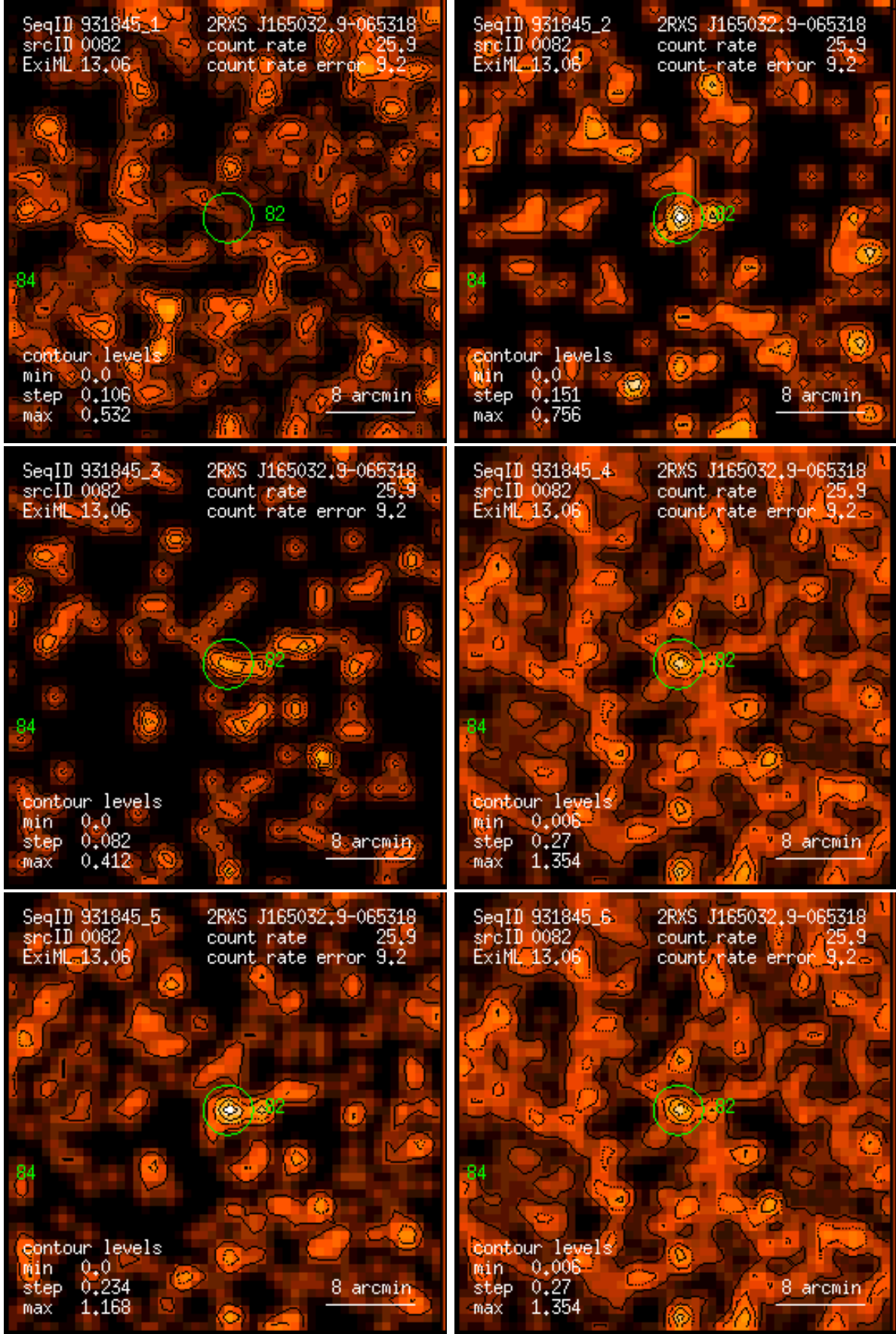
Figure 82: RASS 931845: detection 0082: band rate images, Gaussian filter: (1) PSPC channels 11 – 41, (2) 52 – 90, (3) 91 – 201, (4) 11 – 235, (5) 52 – 201, (6) 11 – 201. Broad band rates in counts/ks. Band rate contour levels in counts/ks/arcmin 2 .
