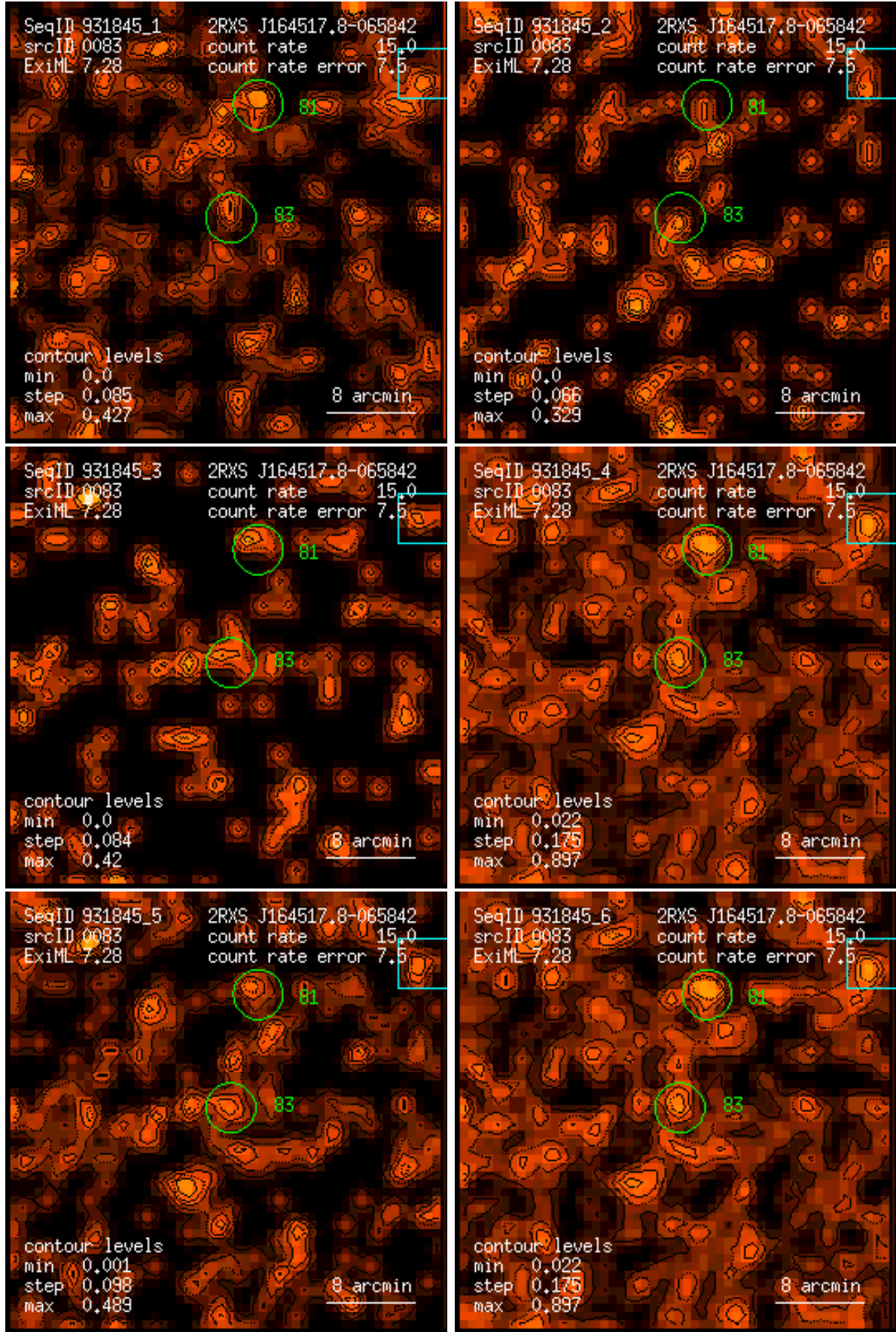
Figure 83: RASS 931845: detection 0083: band rate images, Gaussian filter: (1) PSPC channels 11 – 41, (2) 52 – 90, (3) 91 – 201, (4) 11 – 235, (5) 52 – 201, (6) 11 – 201. Broad band rates in counts/ks. Band rate contour levels in counts/ks/arcmin 2 .
