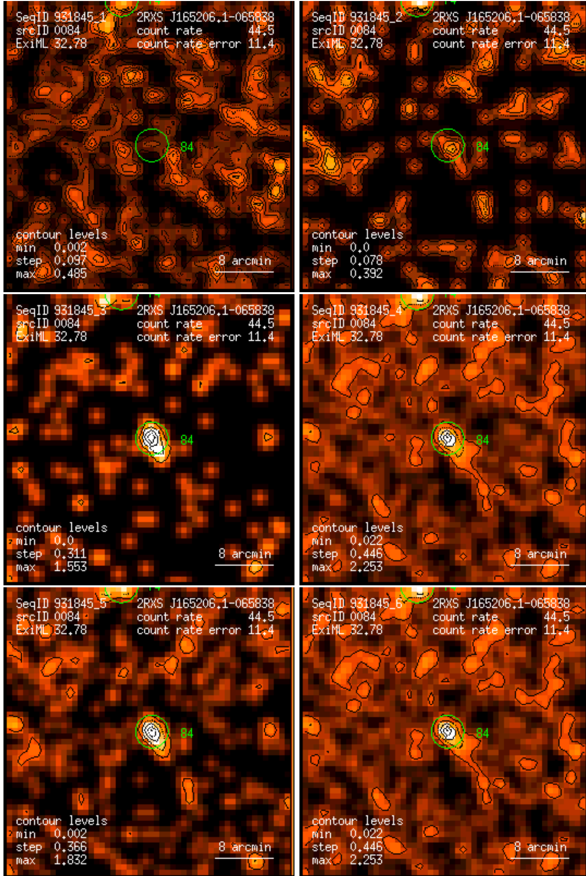
Figure 84: RASS 931845: detection 0084: band rate images, Gaussian filter: (1) PSPC channels 11 – 41, (2) 52 – 90, (3) 91 – 201, (4) 11 – 235, (5) 52 – 201, (6) 11 – 201. Broad band rates in counts/ks. Band rate contour levels in counts/ks/arcmin 2 .
