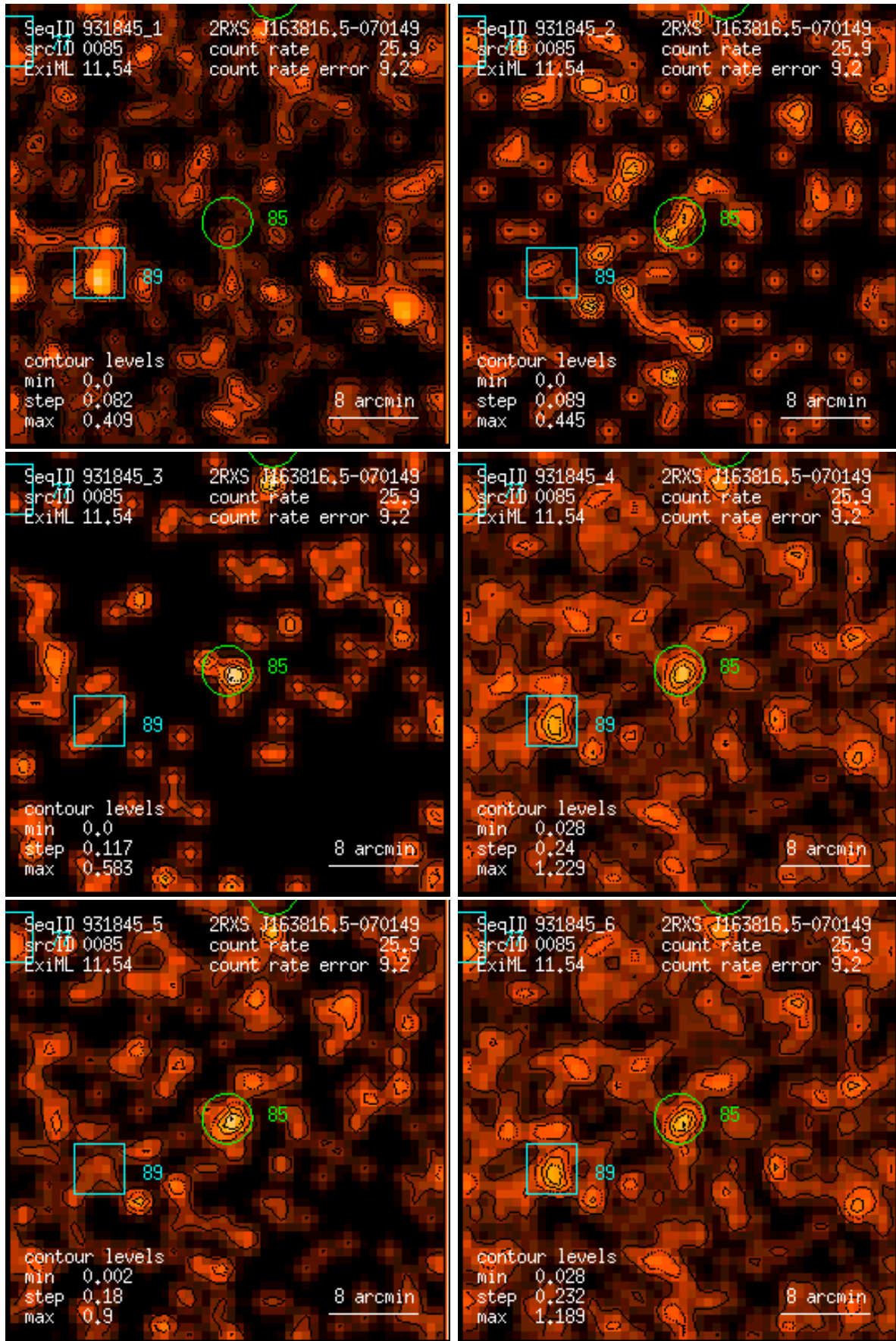
Figure 85: RASS 931845: detection 0085: band rate images, Gaussian filter: (1) PSPC channels 11 – 41, (2) 52 – 90, (3) 91 – 201, (4) 11 – 235, (5) 52 – 201, (6) 11 – 201. Broad band rates in counts/ks. Band rate contour levels in counts/ks/arcmin 2 .
