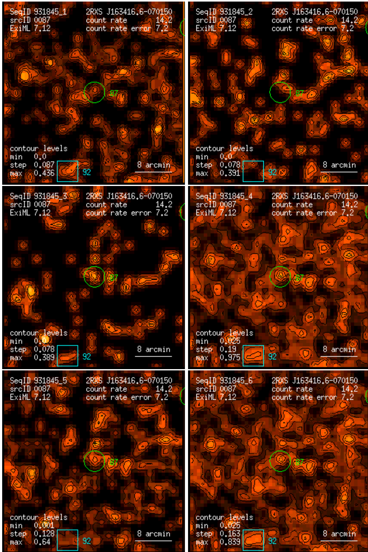
Figure 87: RASS 931845: detection 0087: band rate images, Gaussian filter: (1) PSPC channels 11 – 41, (2) 52 – 90, (3) 91 – 201, (4) 11 – 235, (5) 52 – 201, (6) 11 – 201. Broad band rates in counts/ks. Band rate contour levels in counts/ks/arcmin 2 .
