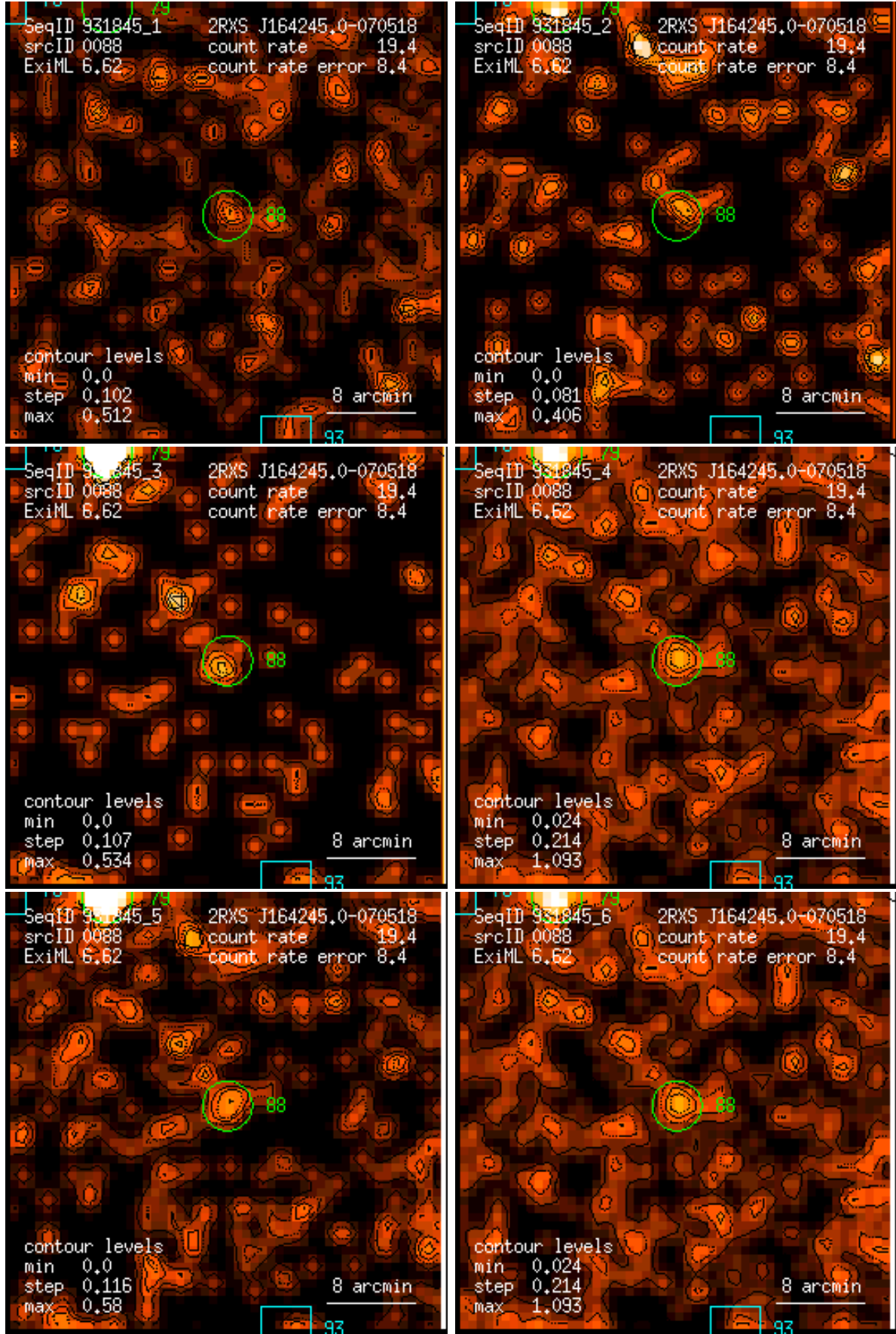
Figure 88: RASS 931845: detection 0088: band rate images, Gaussian filter: (1) PSPC channels 11 – 41, (2) 52 – 90, (3) 91 – 201, (4) 11 – 235, (5) 52 – 201, (6) 11 – 201. Broad band rates in counts/ks. Band rate contour levels in counts/ks/arcmin 2 .
