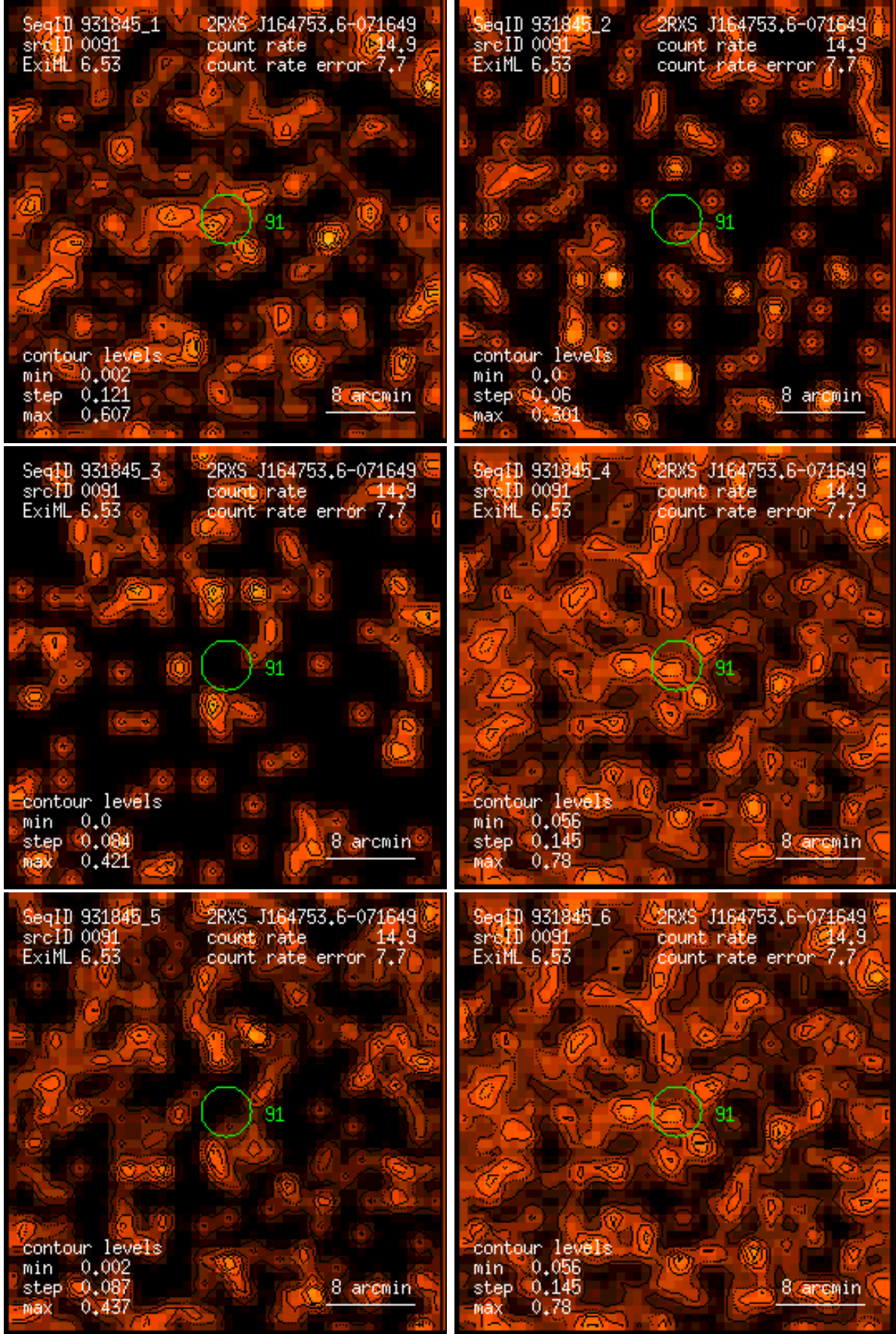
Figure 91: RASS 931845: detection 0091: band rate images, Gaussian filter: (1) PSPC channels 11 – 41, (2) 52 – 90, (3) 91 – 201, (4) 11 – 235, (5) 52 – 201, (6) 11 – 201. Broad band rates in counts/ks. Band rate contour levels in counts/ks/arcmin 2 .
