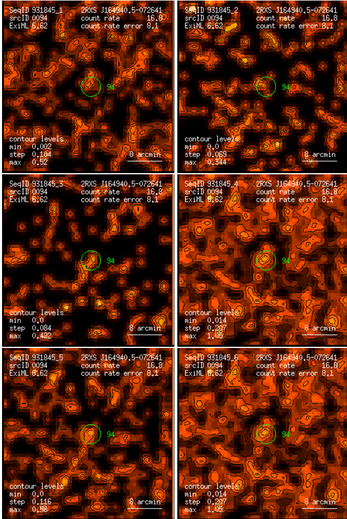
Figure 94: RASS 931845: detection 0094: band rate images, Gaussian filter: (1) PSPC channels 11 – 41, (2) 52 – 90, (3) 91 – 201, (4) 11 – 235, (5) 52 – 201, (6) 11 – 201. Broad band rates in counts/ks. Band rate contour levels in counts/ks/arcmin 2 .
