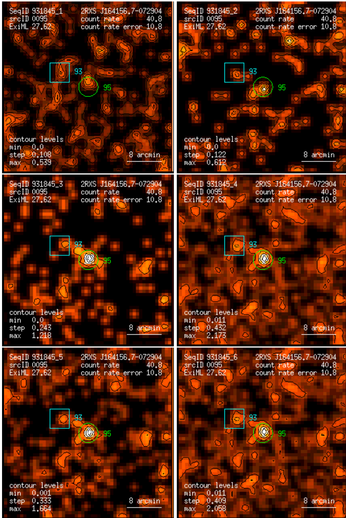
Figure 95: RASS 931845: detection 0095: band rate images, Gaussian filter: (1) PSPC channels 11 – 41, (2) 52 – 90, (3) 91 – 201, (4) 11 – 235, (5) 52 – 201, (6) 11 – 201. Broad band rates in counts/ks. Band rate contour levels in counts/ks/arcmin 2 .
