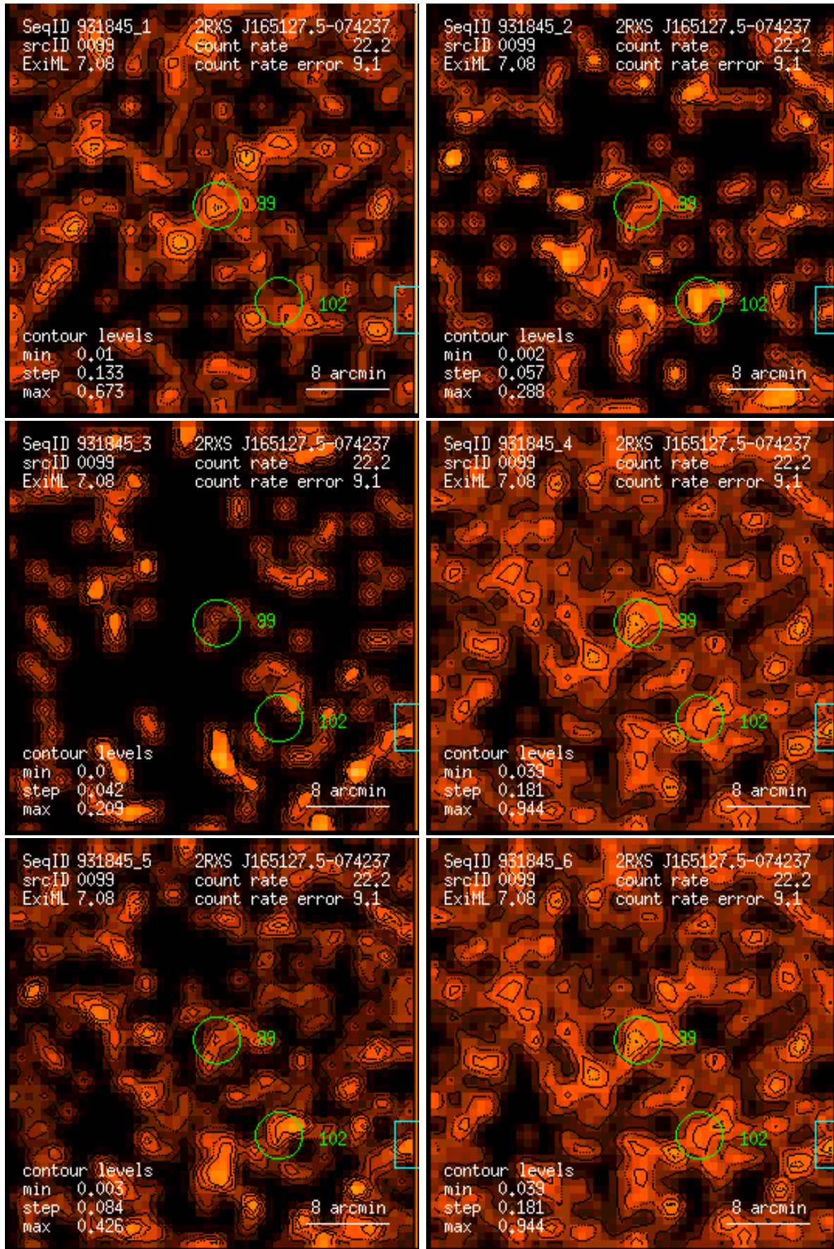
Figure 99: RASS 931845: detection 0099: band rate images, Gaussian filter: (1) PSPC channels 11 – 41, (2) 52 – 90, (3) 91 – 201, (4) 11 – 235, (5) 52 – 201, (6) 11 – 201. Broad band rates in counts/ks. Band rate contour levels in counts/ks/arcmin 2 .
