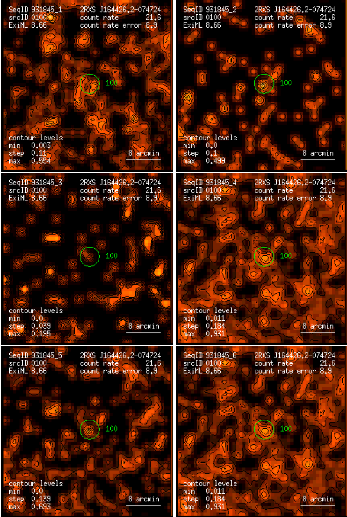
Figure 100: RASS 931845: detection 0100: band rate images, Gaussian filter: (1) PSPC channels 11 – 41, (2) 52 – 90, (3) 91 – 201, (4) 11 – 235, (5) 52 – 201, (6) 11 – 201. Broad band rates in counts/ks. Band rate contour levels in counts/ks/arcmin 2 .
