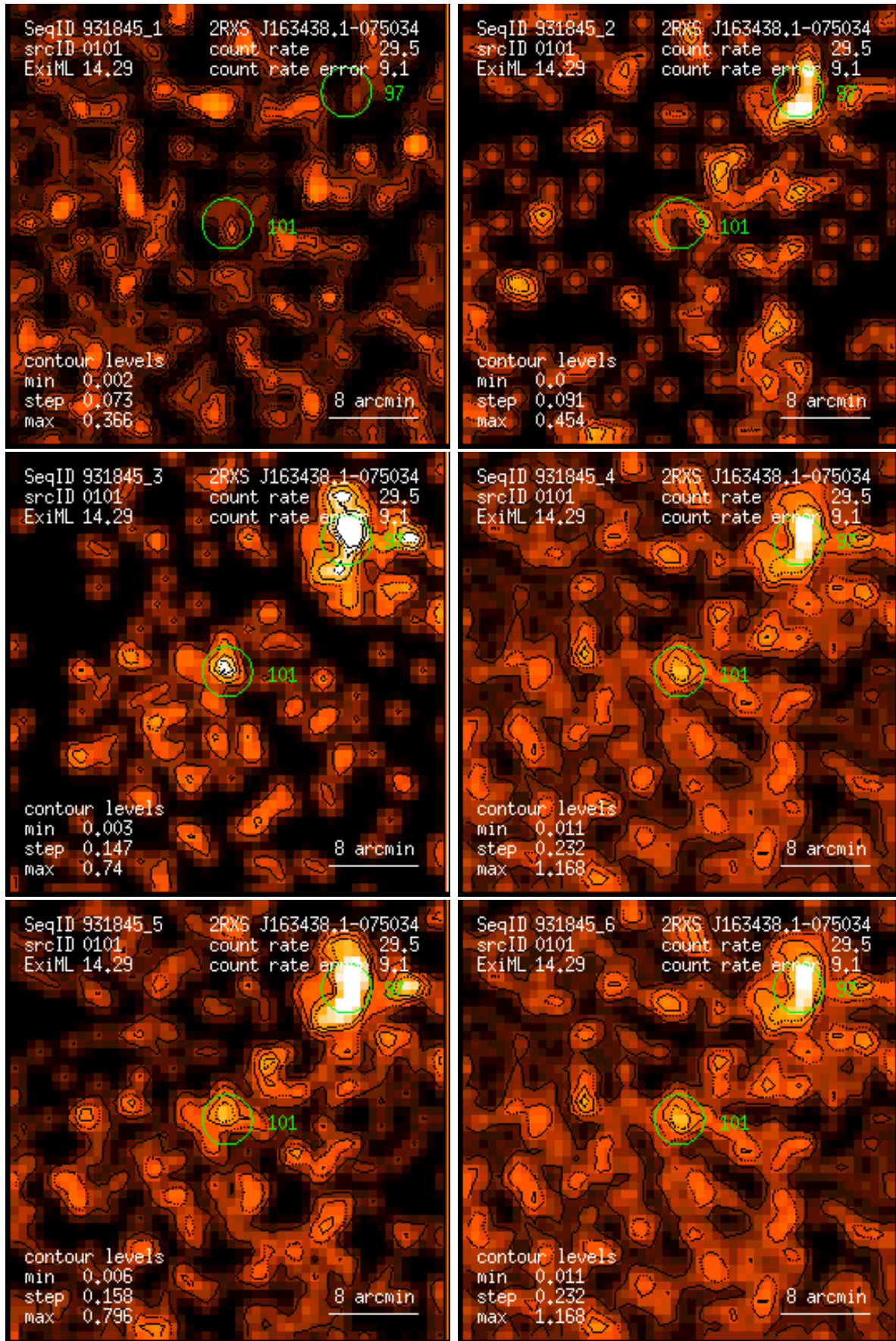
Figure 101: RASS 931845: detection 0101: band rate images, Gaussian filter: (1) PSPC channels 11 – 41, (2) 52 – 90, (3) 91 – 201, (4) 11 – 235, (5) 52 – 201, (6) 11 – 201. Broad band rates in counts/ks. Band rate contour levels in counts/ks/arcmin 2 .
