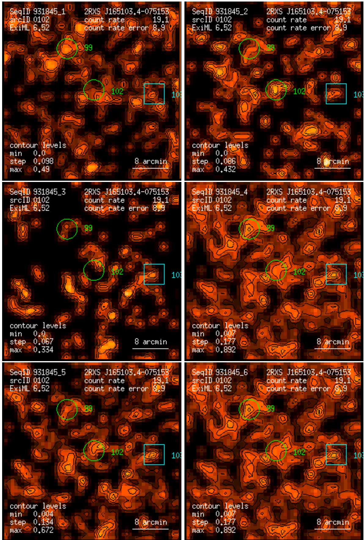
Figure 102: RASS 931845: detection 0102: band rate images, Gaussian filter: (1) PSPC channels 11 – 41, (2) 52 – 90, (3) 91 – 201, (4) 11 – 235, (5) 52 – 201, (6) 11 – 201. Broad band rates in counts/ks. Band rate contour levels in counts/ks/arcmin 2 .
