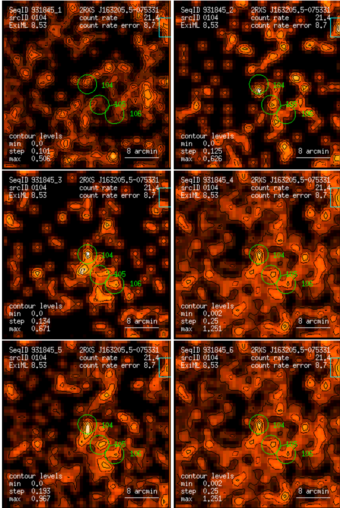
Figure 104: RASS 931845: detection 0104: band rate images, Gaussian filter: (1) PSPC channels 11 – 41, (2) 52 – 90, (3) 91 – 201, (4) 11 – 235, (5) 52 – 201, (6) 11 – 201. Broad band rates in counts/ks. Band rate contour levels in counts/ks/arcmin 2 .
