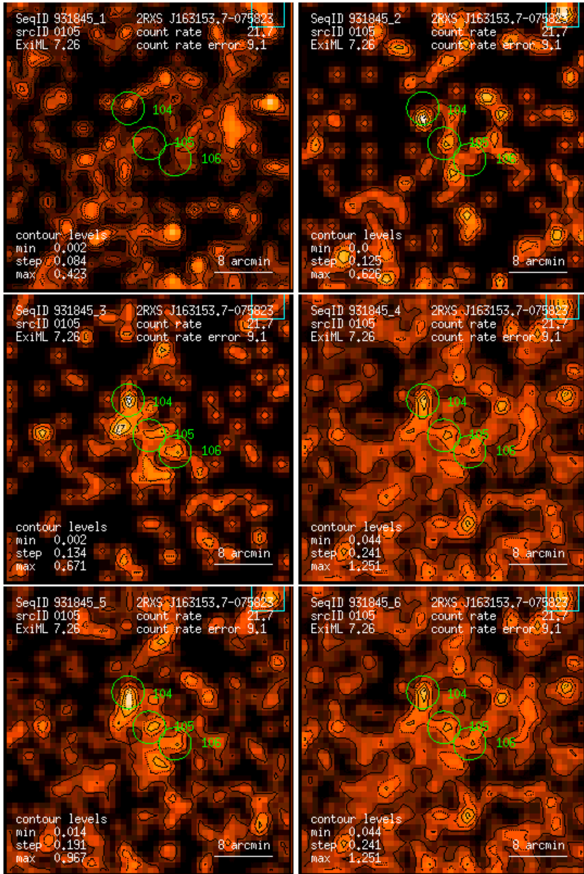
Figure 105: RASS 931845: detection 0105: band rate images, Gaussian filter: (1) PSPC channels 11 – 41, (2) 52 – 90, (3) 91 – 201, (4) 11 – 235, (5) 52 – 201, (6) 11 – 201. Broad band rates in counts/ks. Band rate contour levels in counts/ks/arcmin 2 .
