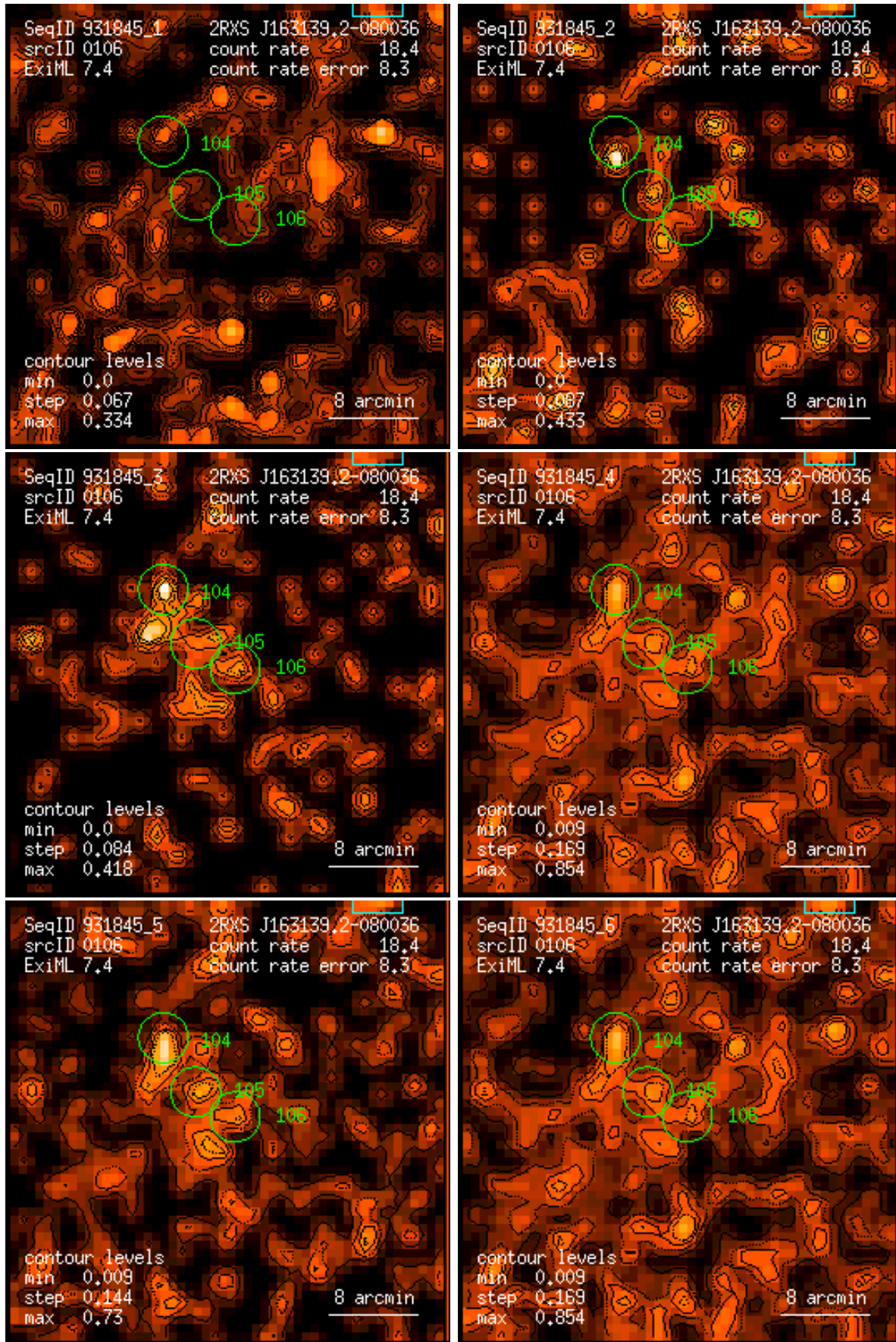
Figure 106: RASS 931845: detection 0106: band rate images, Gaussian filter: (1) PSPC channels 11 – 41, (2) 52 – 90, (3) 91 – 201, (4) 11 – 235, (5) 52 – 201, (6) 11 – 201. Broad band rates in counts/ks. Band rate contour levels in counts/ks/arcmin 2 .
