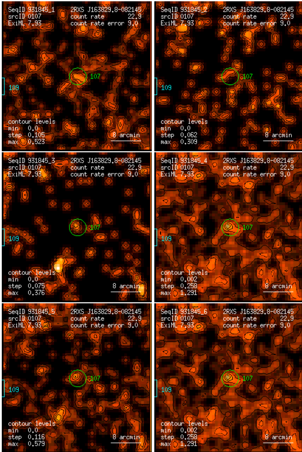
Figure 107: RASS 931845: detection 0107: band rate images, Gaussian filter: (1) PSPC channels 11 – 41, (2) 52 – 90, (3) 91 – 201, (4) 11 – 235, (5) 52 – 201, (6) 11 – 201. Broad band rates in counts/ks. Band rate contour levels in counts/ks/arcmin 2 .
