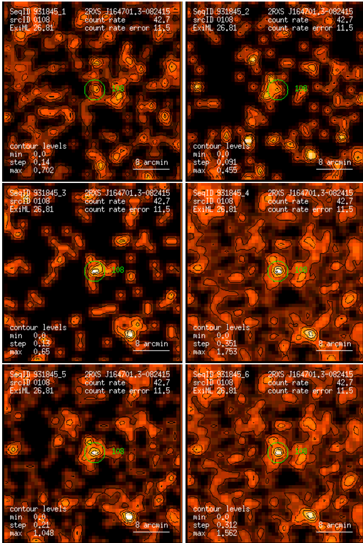
Figure 108: RASS 931845: detection 0108: band rate images, Gaussian filter: (1) PSPC channels 11 – 41, (2) 52 – 90, (3) 91 – 201, (4) 11 – 235, (5) 52 – 201, (6) 11 – 201. Broad band rates in counts/ks. Band rate contour levels in counts/ks/arcmin 2 .
