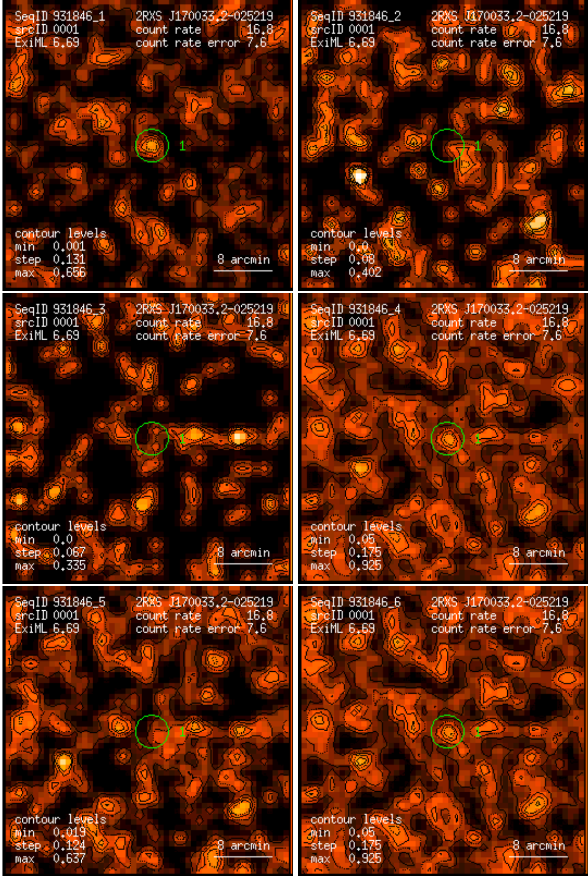
Figure 1: RASS 931846: detection 0001: band rate images, Gaussian filter: (1) PSPC channels 11 – 41, (2) 52 – 90, (3) 91 – 201, (4) 11 – 235, (5) 52 – 201, (6) 11 – 201. Broad band rates in counts/ks. Band rate contour levels in counts/ks/arcmin 2 .
