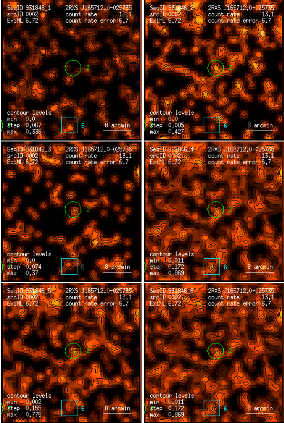
Figure 2: RASS 931846: detection 0002: band rate images, Gaussian filter: (1) PSPC channels 11 – 41, (2) 52 – 90, (3) 91 – 201, (4) 11 – 235, (5) 52 – 201, (6) 11 – 201. Broad band rates in counts/ks. Band rate contour levels in counts/ks/arcmin 2 .
