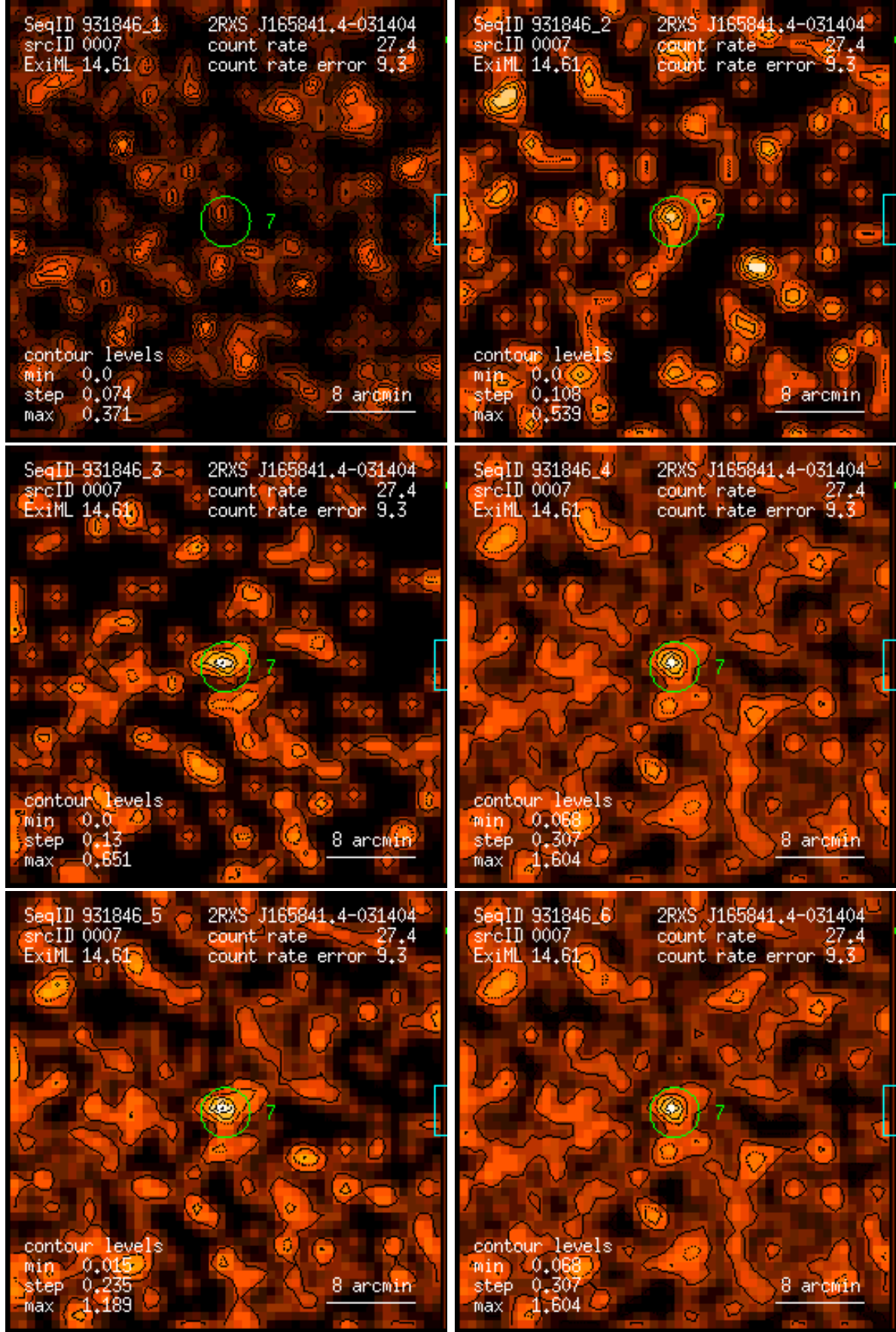
Figure 7: RASS 931846: detection 0007: band rate images, Gaussian filter: (1) PSPC channels 11 – 41, (2) 52 – 90, (3) 91 – 201, (4) 11 – 235, (5) 52 – 201, (6) 11 – 201. Broad band rates in counts/ks. Band rate contour levels in counts/ks/arcmin 2 .
