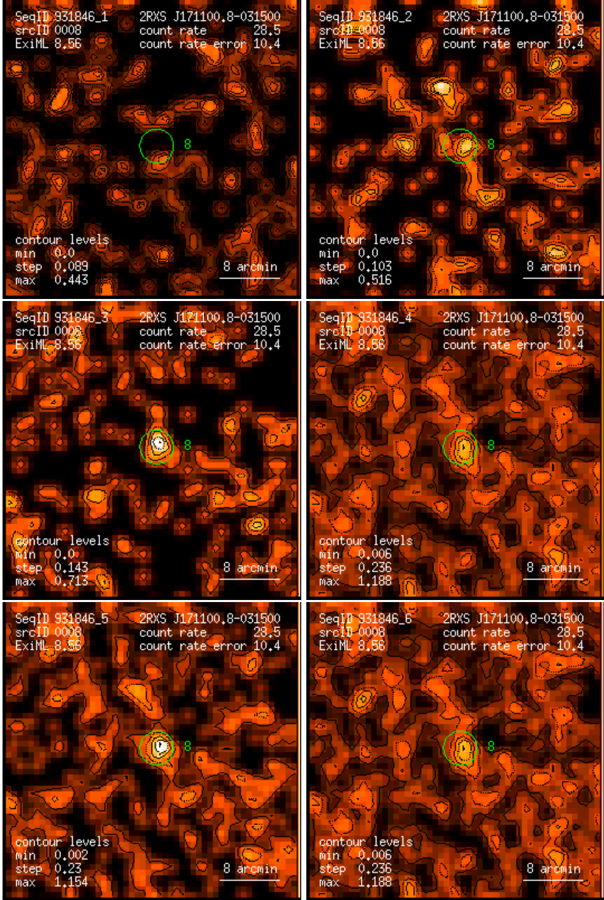
Figure 8: RASS 931846: detection 0008: band rate images, Gaussian filter: (1) PSPC channels 11 – 41, (2) 52 – 90, (3) 91 – 201, (4) 11 – 235, (5) 52 – 201, (6) 11 – 201. Broad band rates in counts/ks. Band rate contour levels in counts/ks/arcmin 2 .
