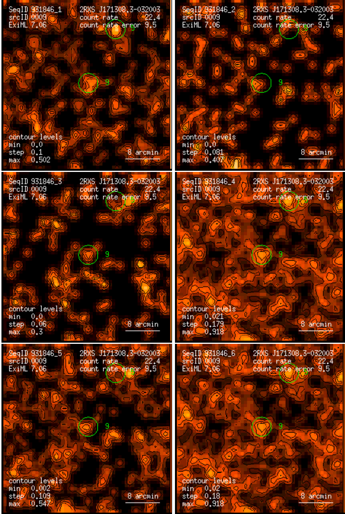
Figure 9: RASS 931846: detection 0009: band rate images, Gaussian filter: (1) PSPC channels 11 – 41, (2) 52 – 90, (3) 91 – 201, (4) 11 – 235, (5) 52 – 201, (6) 11 – 201. Broad band rates in counts/ks. Band rate contour levels in counts/ks/arcmin 2 .
