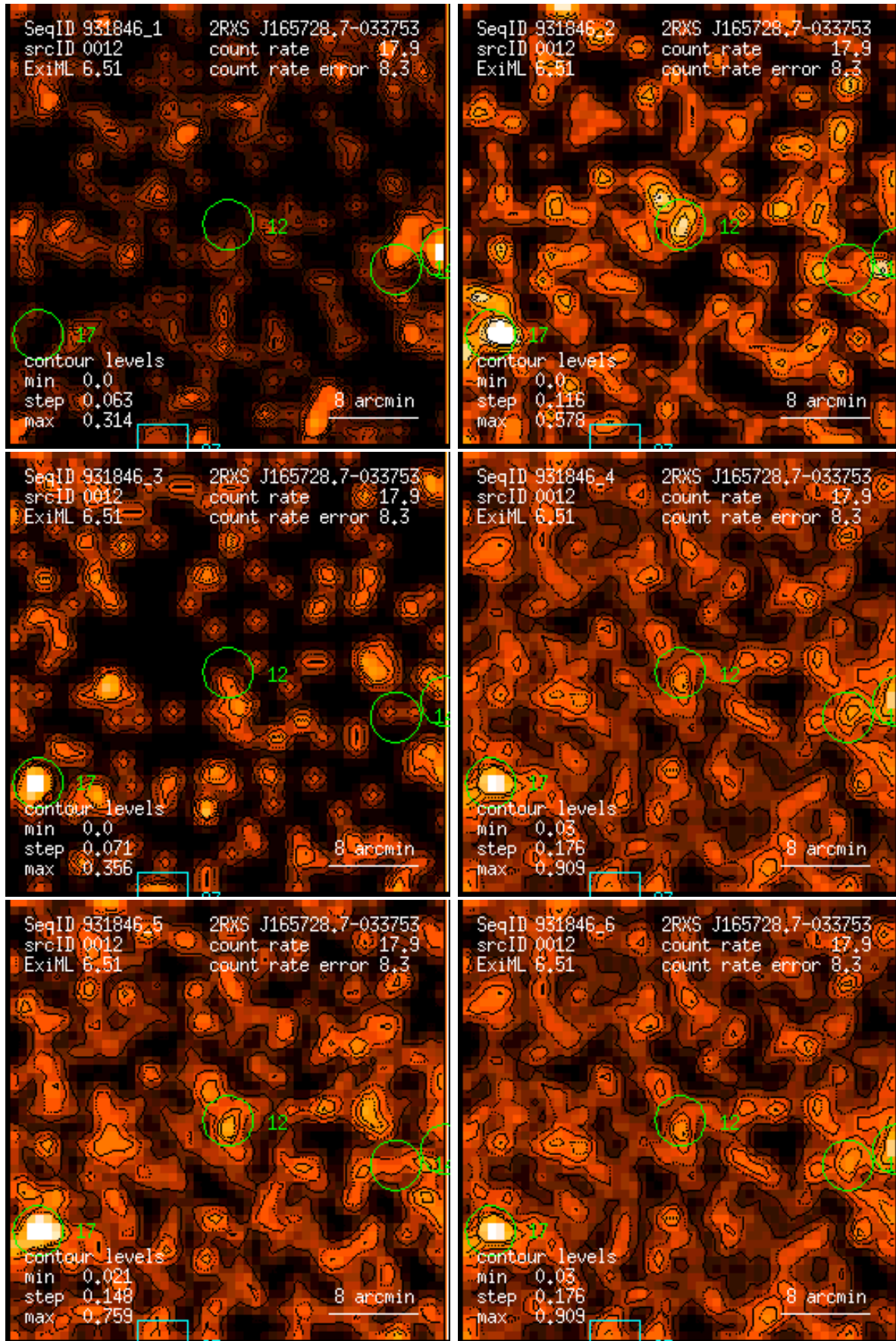
Figure 12: RASS 931846: detection 0012: band rate images, Gaussian filter: (1) PSPC channels 11 – 41, (2) 52 – 90, (3) 91 – 201, (4) 11 – 235, (5) 52 – 201, (6) 11 – 201. Broad band rates in counts/ks. Band rate contour levels in counts/ks/arcmin 2 .
