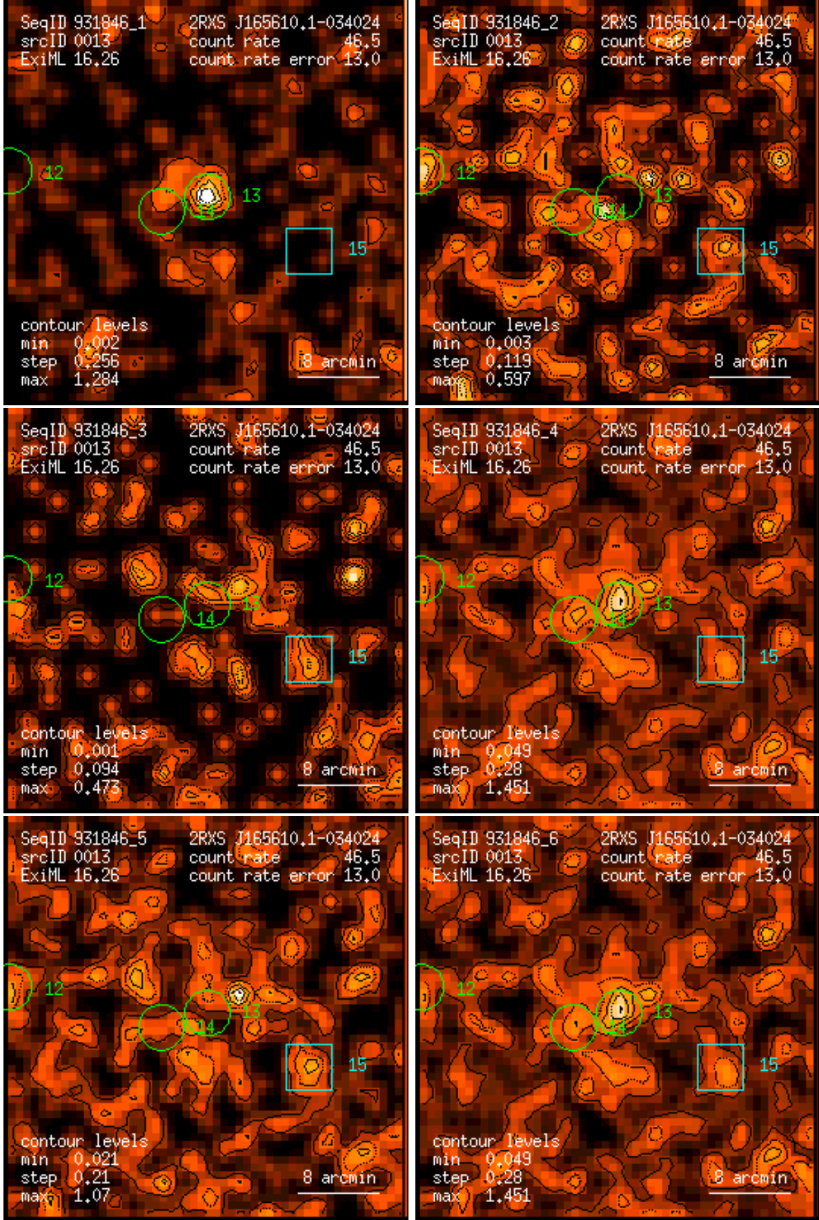
Figure 13: RASS 931846: detection 0013: band rate images, Gaussian filter: (1) PSPC channels 11 – 41, (2) 52 – 90, (3) 91 – 201, (4) 11 – 235, (5) 52 – 201, (6) 11 – 201. Broad band rates in counts/ks. Band rate contour levels in counts/ks/arcmin 2 .
