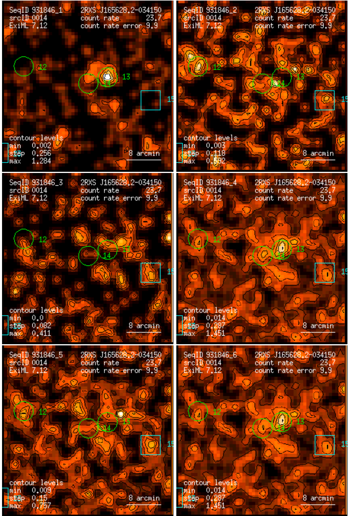
Figure 14: RASS 931846: detection 0014: band rate images, Gaussian filter: (1) PSPC channels 11 – 41, (2) 52 – 90, (3) 91 – 201, (4) 11 – 235, (5) 52 – 201, (6) 11 – 201. Broad band rates in counts/ks. Band rate contour levels in counts/ks/arcmin 2 .
