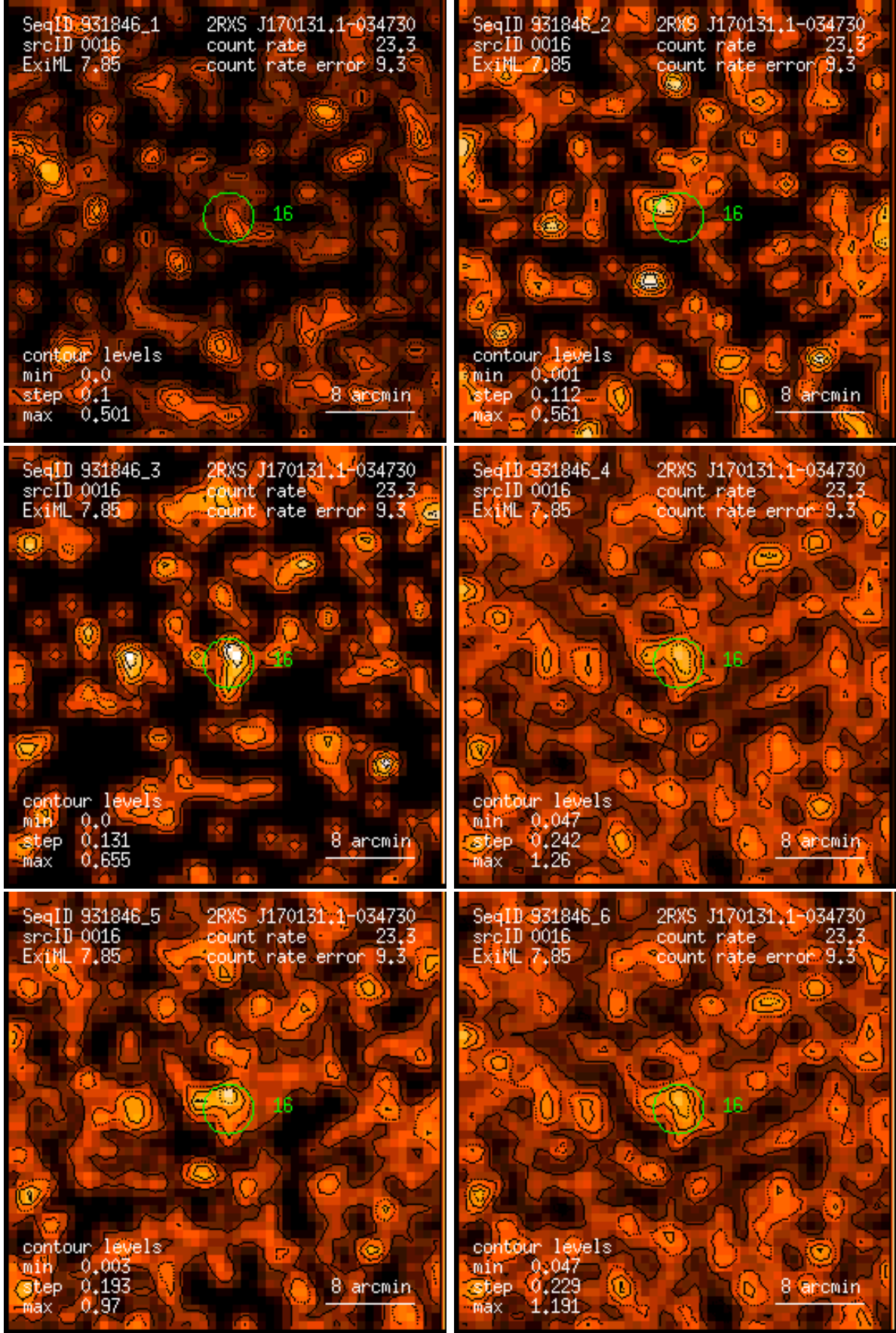
Figure 16: RASS 931846: detection 0016: band rate images, Gaussian filter: (1) PSPC channels 11 – 41, (2) 52 – 90, (3) 91 – 201, (4) 11 – 235, (5) 52 – 201, (6) 11 – 201. Broad band rates in counts/ks. Band rate contour levels in counts/ks/arcmin 2 .
