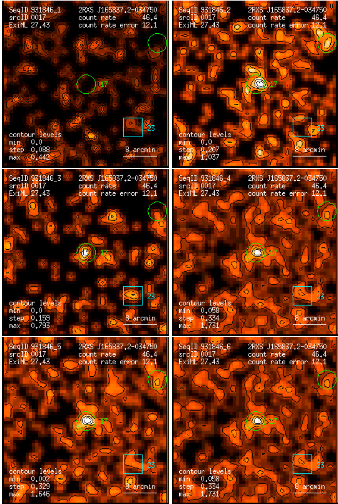
Figure 17: RASS 931846: detection 0017: band rate images, Gaussian filter: (1) PSPC channels 11 – 41, (2) 52 – 90, (3) 91 – 201, (4) 11 – 235, (5) 52 – 201, (6) 11 – 201. Broad band rates in counts/ks. Band rate contour levels in counts/ks/arcmin 2 .
