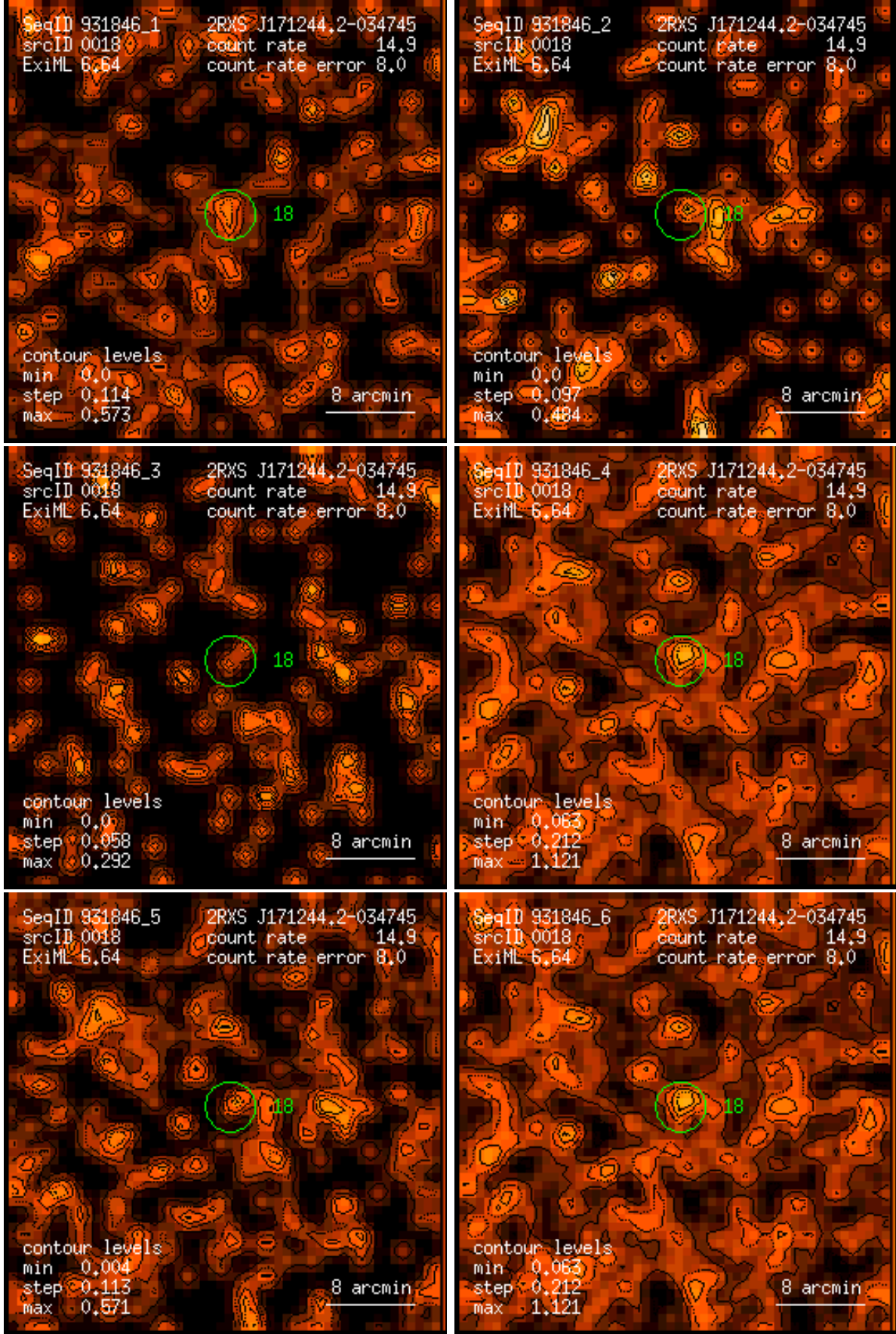
Figure 18: RASS 931846: detection 0018: band rate images, Gaussian filter: (1) PSPC channels 11 – 41, (2) 52 – 90, (3) 91 – 201, (4) 11 – 235, (5) 52 – 201, (6) 11 – 201. Broad band rates in counts/ks. Band rate contour levels in counts/ks/arcmin 2 .
