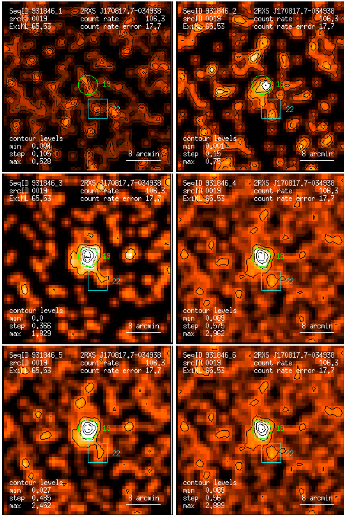
Figure 19: RASS 931846: detection 0019: band rate images, Gaussian filter: (1) PSPC channels 11 – 41, (2) 52 – 90, (3) 91 – 201, (4) 11 – 235, (5) 52 – 201, (6) 11 – 201. Broad band rates in counts/ks. Band rate contour levels in counts/ks/arcmin 2 .
