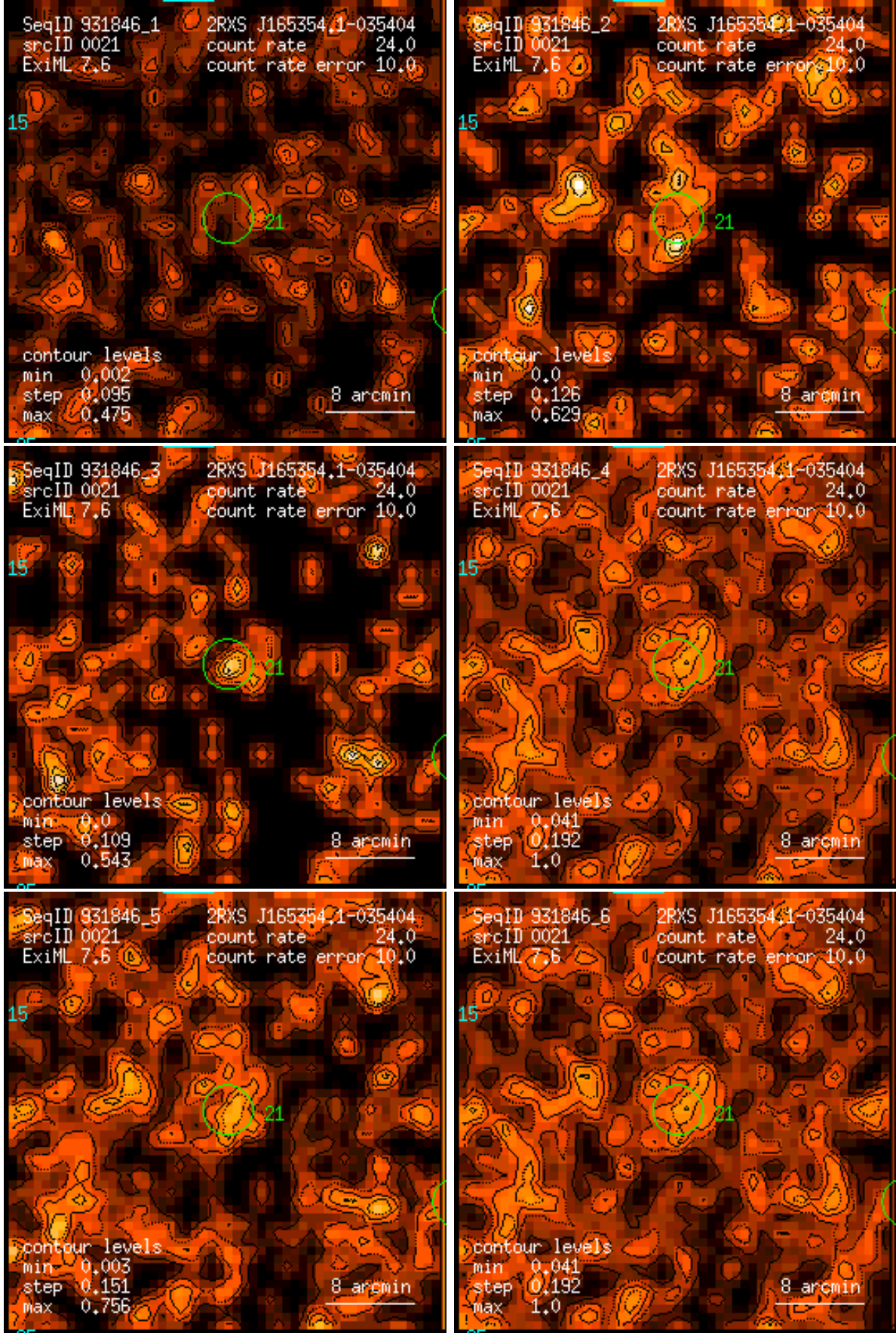
Figure 21: RASS 931846: detection 0021: band rate images, Gaussian filter: (1) PSPC channels 11 – 41, (2) 52 – 90, (3) 91 – 201, (4) 11 – 235, (5) 52 – 201, (6) 11 – 201. Broad band rates in counts/ks. Band rate contour levels in counts/ks/arcmin 2 .
