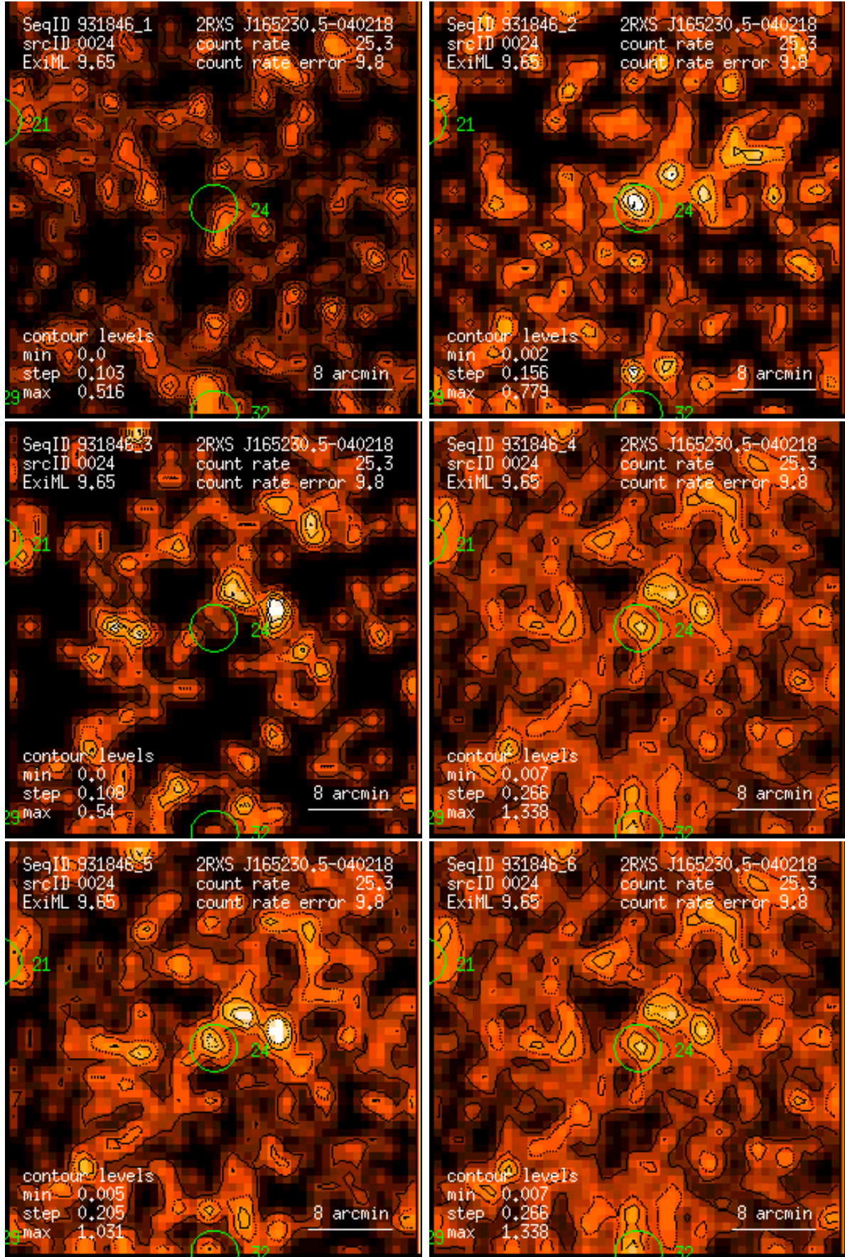
Figure 24: RASS 931846: detection 0024: band rate images, Gaussian filter: (1) PSPC channels 11 – 41, (2) 52 – 90, (3) 91 – 201, (4) 11 – 235, (5) 52 – 201, (6) 11 – 201. Broad band rates in counts/ks. Band rate contour levels in counts/ks/arcmin 2 .
