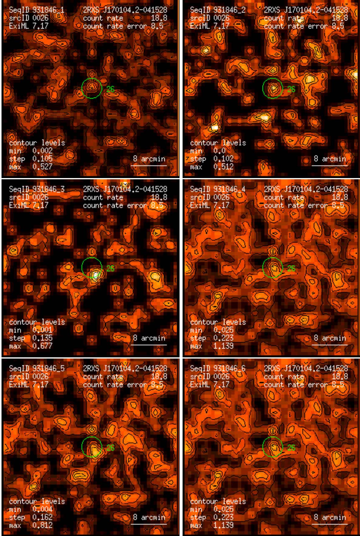
Figure 26: RASS 931846: detection 0026: band rate images, Gaussian filter: (1) PSPC channels 11 – 41, (2) 52 – 90, (3) 91 – 201, (4) 11 – 235, (5) 52 – 201, (6) 11 – 201. Broad band rates in counts/ks. Band rate contour levels in counts/ks/arcmin 2 .
