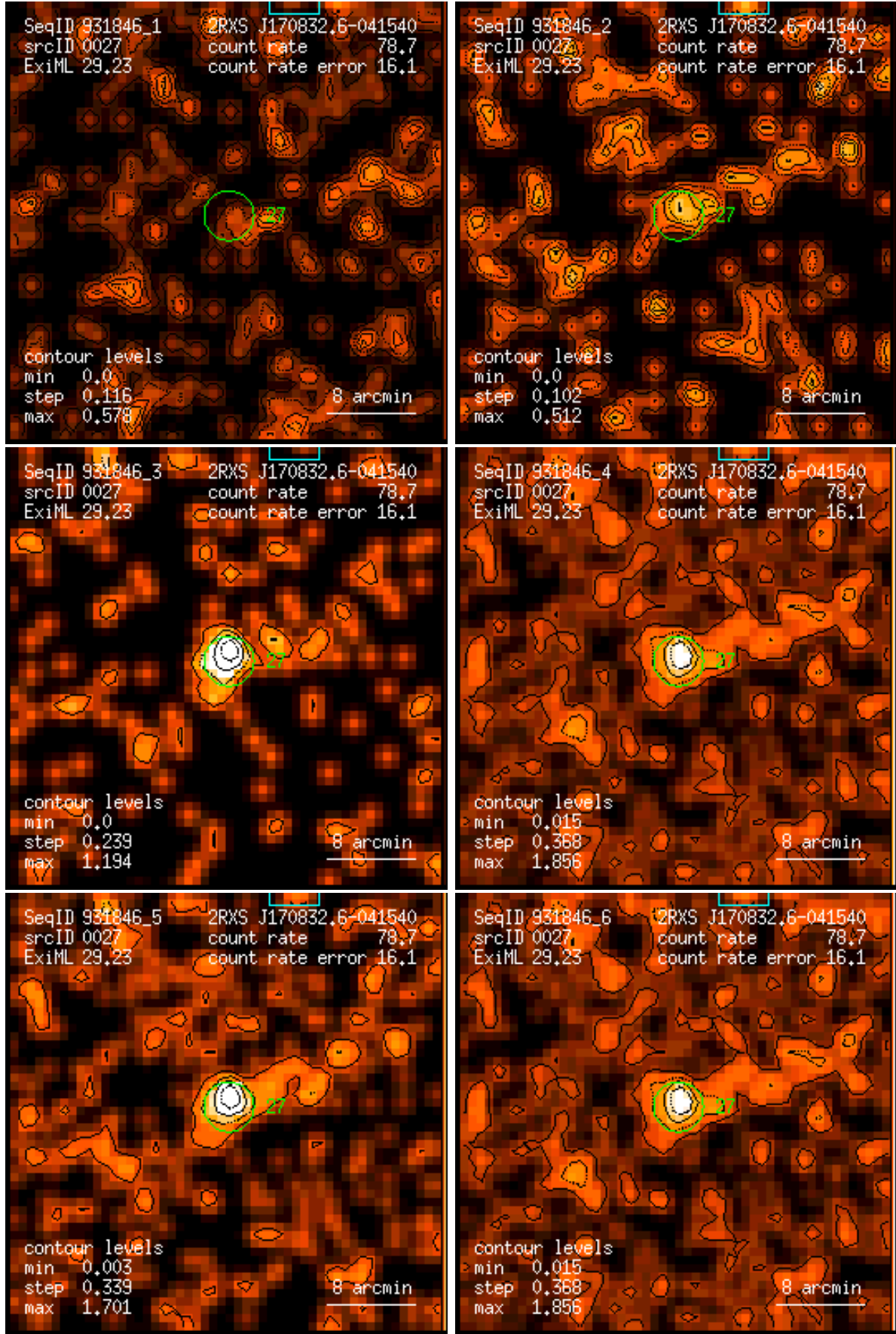
Figure 27: RASS 931846: detection 0027: band rate images, Gaussian filter: (1) PSPC channels 11 – 41, (2) 52 – 90, (3) 91 – 201, (4) 11 – 235, (5) 52 – 201, (6) 11 – 201. Broad band rates in counts/ks. Band rate contour levels in counts/ks/arcmin 2 .
