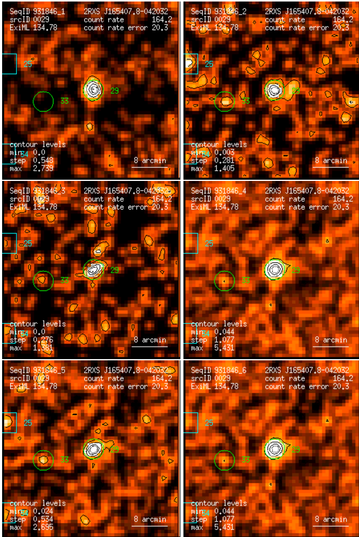
Figure 29: RASS 931846: detection 0029: band rate images, Gaussian filter: (1) PSPC channels 11 – 41, (2) 52 – 90, (3) 91 – 201, (4) 11 – 235, (5) 52 – 201, (6) 11 – 201. Broad band rates in counts/ks. Band rate contour levels in counts/ks/arcmin 2 .
