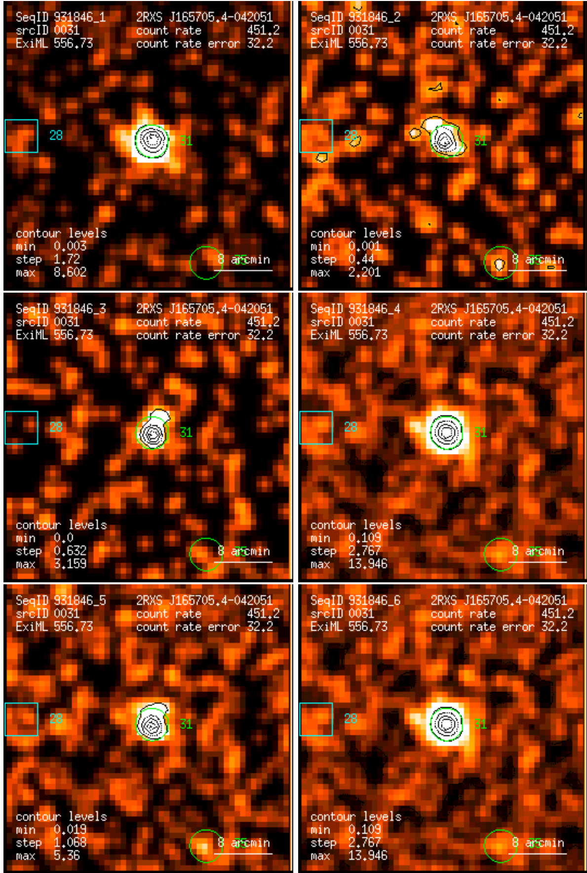
Figure 31: RASS 931846: detection 0031: band rate images, Gaussian filter: (1) PSPC channels 11 – 41, (2) 52 – 90, (3) 91 – 201, (4) 11 – 235, (5) 52 – 201, (6) 11 – 201. Broad band rates in counts/ks. Band rate contour levels in counts/ks/arcmin 2 .
