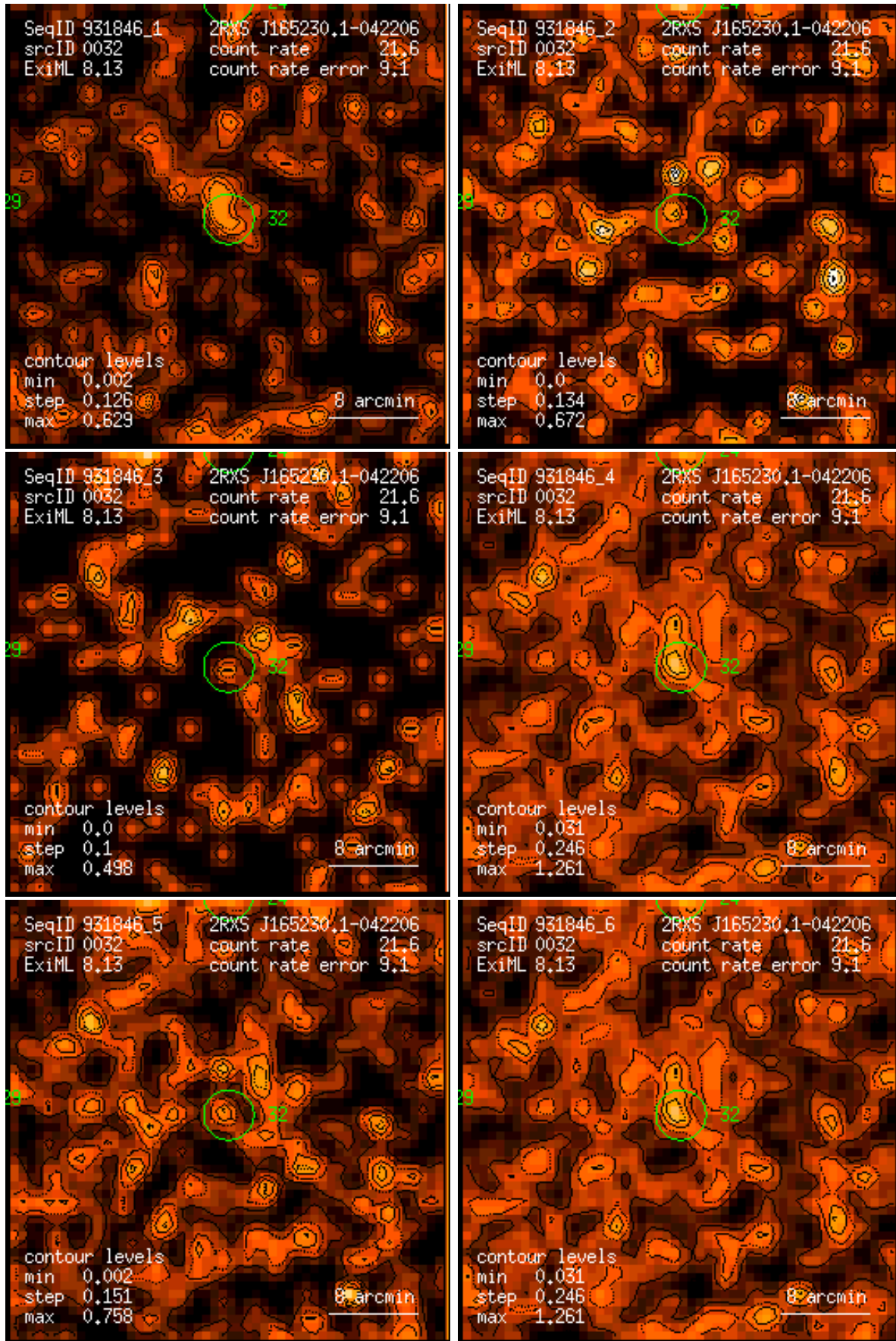
Figure 32: RASS 931846: detection 0032: band rate images, Gaussian filter: (1) PSPC channels 11 – 41, (2) 52 – 90, (3) 91 – 201, (4) 11 – 235, (5) 52 – 201, (6) 11 – 201. Broad band rates in counts/ks. Band rate contour levels in counts/ks/arcmin 2 .
