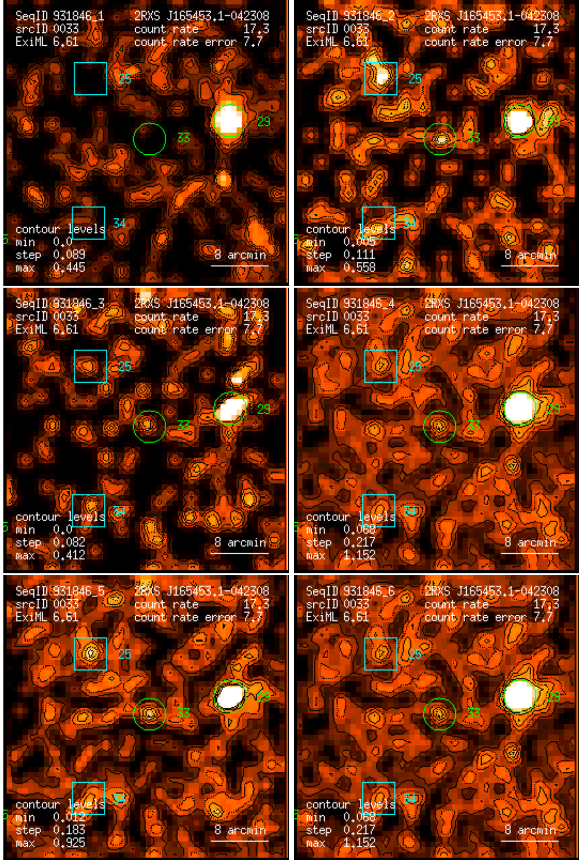
Figure 33: RASS 931846: detection 0033: band rate images, Gaussian filter: (1) PSPC channels 11 – 41, (2) 52 – 90, (3) 91 – 201, (4) 11 – 235, (5) 52 – 201, (6) 11 – 201. Broad band rates in counts/ks. Band rate contour levels in counts/ks/arcmin 2 .
