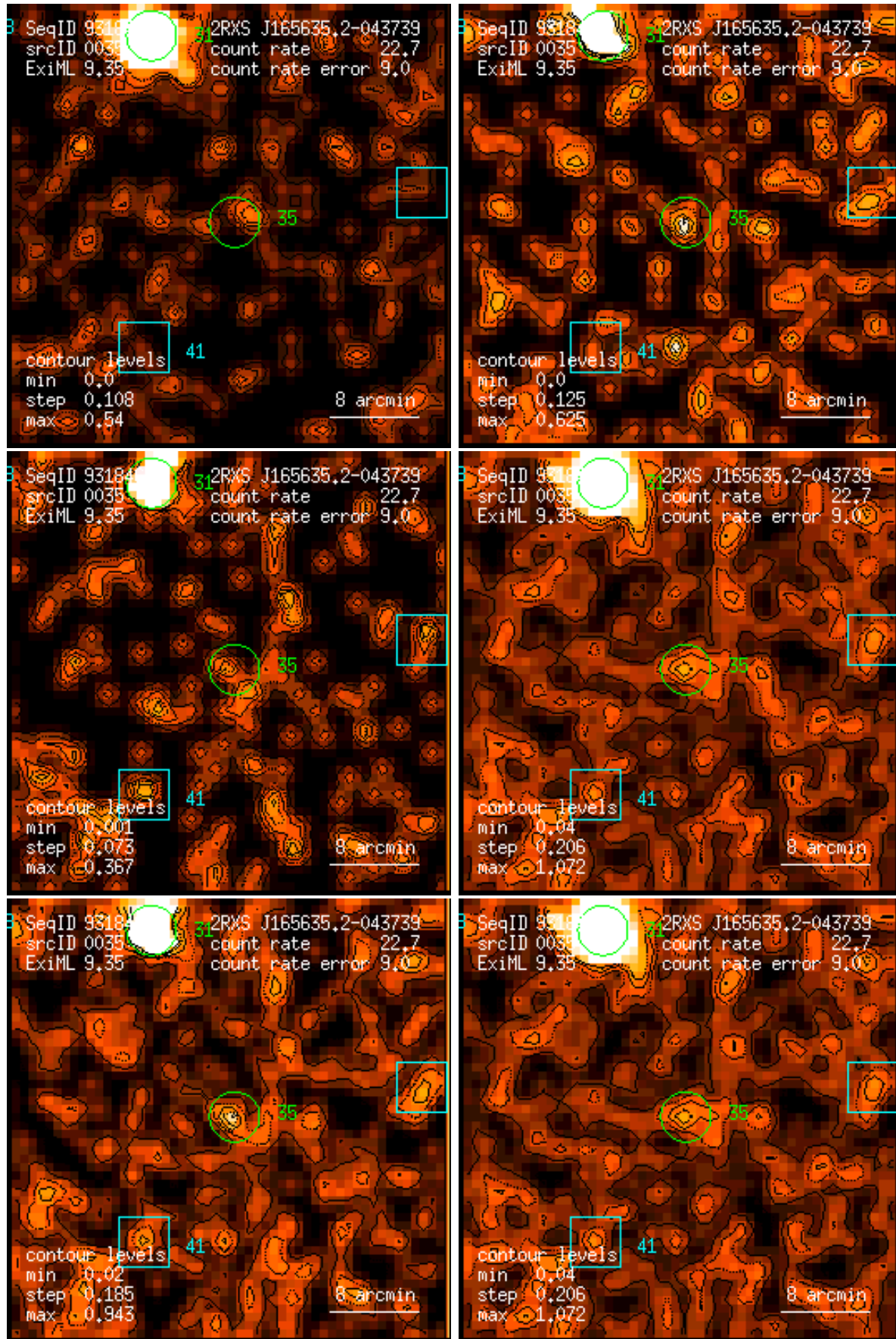
Figure 35: RASS 931846: detection 0035: band rate images, Gaussian filter: (1) PSPC channels 11 – 41, (2) 52 – 90, (3) 91 – 201, (4) 11 – 235, (5) 52 – 201, (6) 11 – 201. Broad band rates in counts/ks. Band rate contour levels in counts/ks/arcmin 2 .
