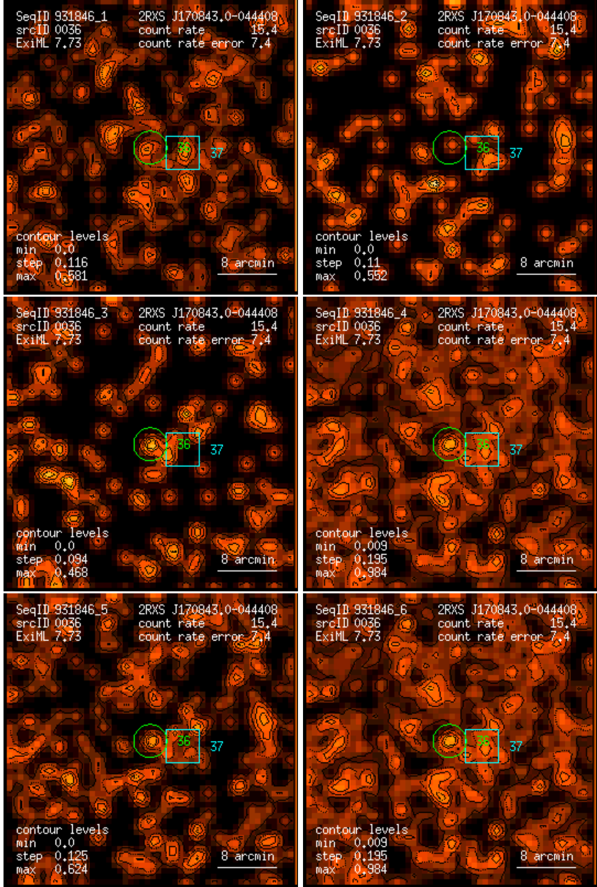
Figure 36: RASS 931846: detection 0036: band rate images, Gaussian filter: (1) PSPC channels 11 – 41, (2) 52 – 90, (3) 91 – 201, (4) 11 – 235, (5) 52 – 201, (6) 11 – 201. Broad band rates in counts/ks. Band rate contour levels in counts/ks/arcmin 2 .
