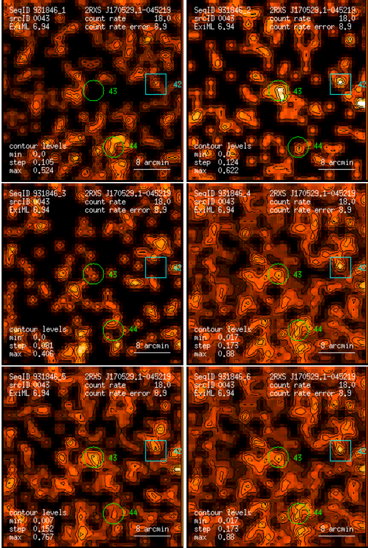
Figure 43: RASS 931846: detection 0043: band rate images, Gaussian filter: (1) PSPC channels 11 – 41, (2) 52 – 90, (3) 91 – 201, (4) 11 – 235, (5) 52 – 201, (6) 11 – 201. Broad band rates in counts/ks. Band rate contour levels in counts/ks/arcmin 2 .
